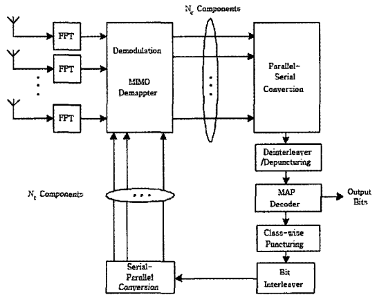
Figure 2. Receiver structure for ST-BICM-OFDM with UEP.
