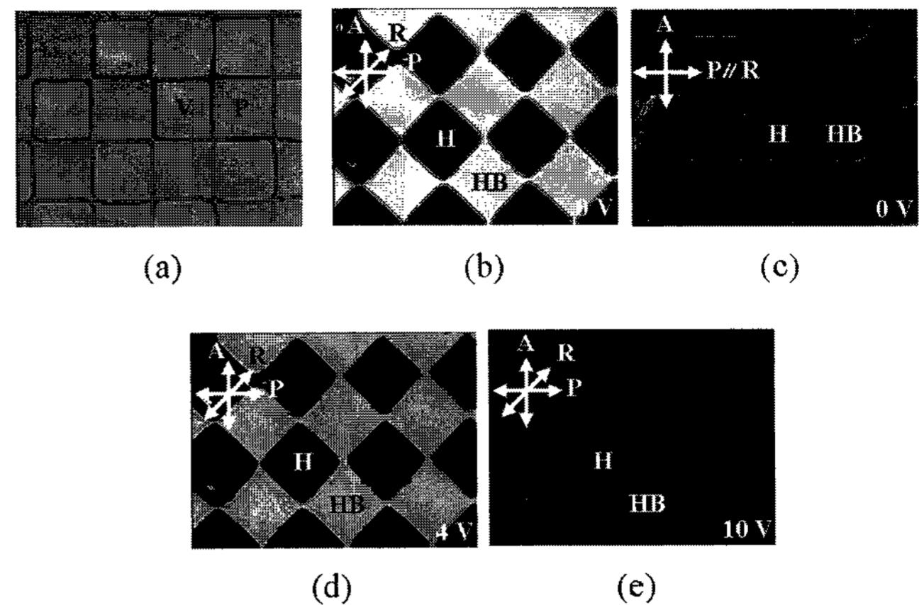
Fig. 5. (a) The microscopic image of the patterned homeotropic LC alignment PI (AL1H659) layer on the planar LC alignment PI (RN1199) layer. (b), (c), (d), and (e) are the polarizing microscopic images of the LC ( \Delta\epsilon > 0 ) cell with two domains of the homeotropic (H) and the hybrid (HB) geometries, which is produced by assembling the patterned substrate of (a) with the other substrate uniformly coated by the homeotropic LC alignment layer. (b) and (c) are obtained in the absence of an applied voltage. (d) and (e) are obtained in the presence of applied voltages of 4 V and 10 V, respectively.
