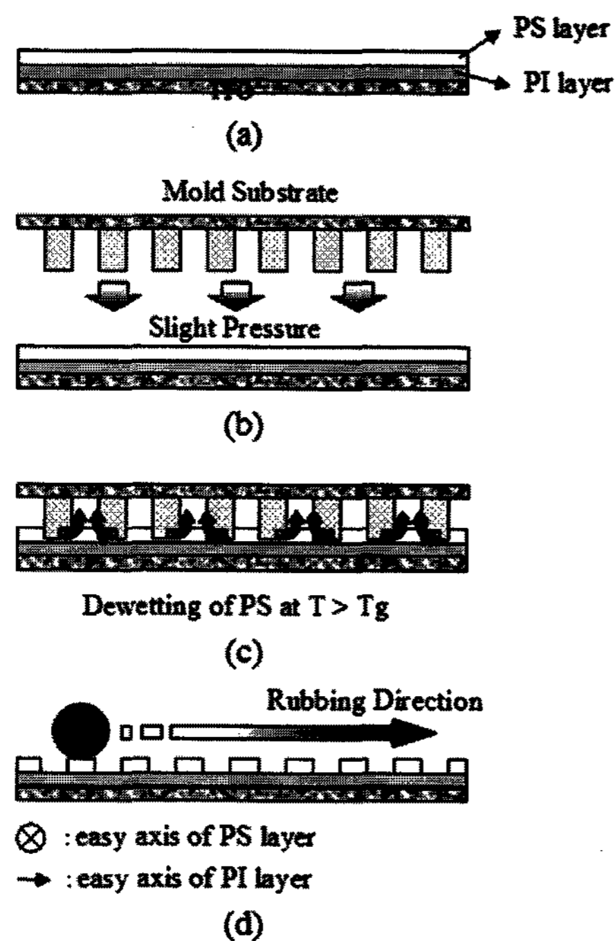
Fig. 6. Schematic of pressure-assisted capillary force lithographic procedures for patterning LC alignment layers.
