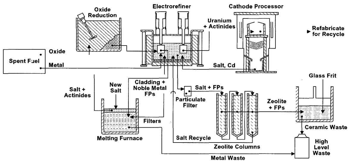
Fig. 10. Pyroprocessing Flowsheet
