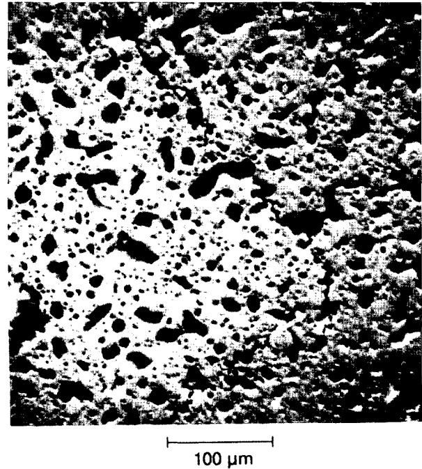
Fig. 2. Fission Gas Pore Morphology of Irradiated U-10Zr Fuel
