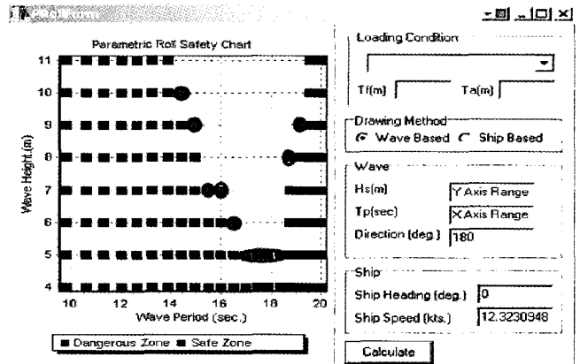
Fig. 8. Parametric Roll Stability Chart.
