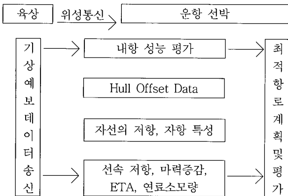
Fig. 1. Configuration of Optimum Navigation Route Safety Assessment System.
