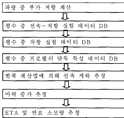
Fig. 9. Flow chart of speed reduction / Power increase estimation.
