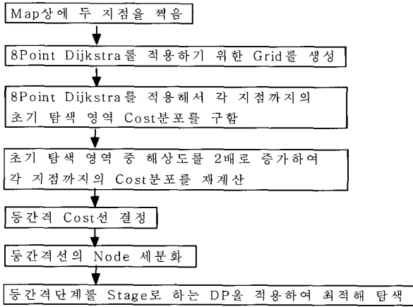
Fig. 12. Flow Chart of Optimum Route Search.
