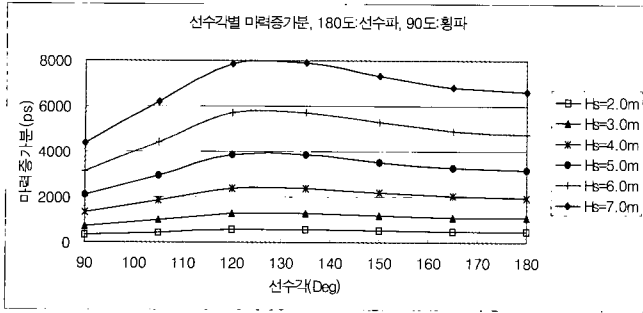
Fig. 11. Power increase according to ship heading.
