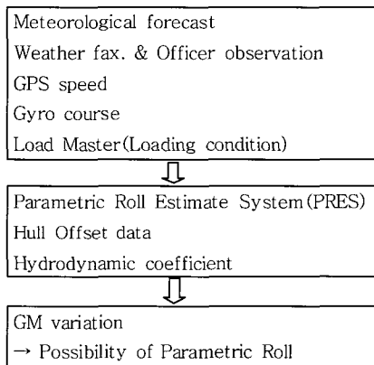
Fig. 6. Configuration of Parametric Roll System.
