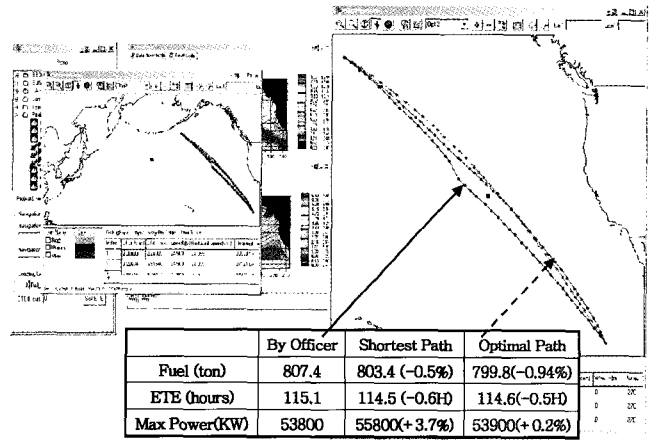
Fig. 14. Result of Three Alternative Routes.
