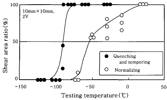
Fig. 1 Charpy impact property of weld seam of X65-grade ERW line pipe 3)
