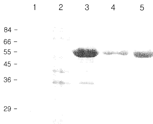
Fig. 1. SDS-PAGE analysis of the stages of the purification of the AHAS III large subunits on 12% polyacrylamide gels. Lane 1, Molecular weight markers; Lane 2 and 3, protein before induction with 0.4 mM IPTG and after induction respectively; Lane 4, AHAS from the elution fraction of Ni-NTA column; Lane 5, AHAS from the elution fraction of gel filtration.
