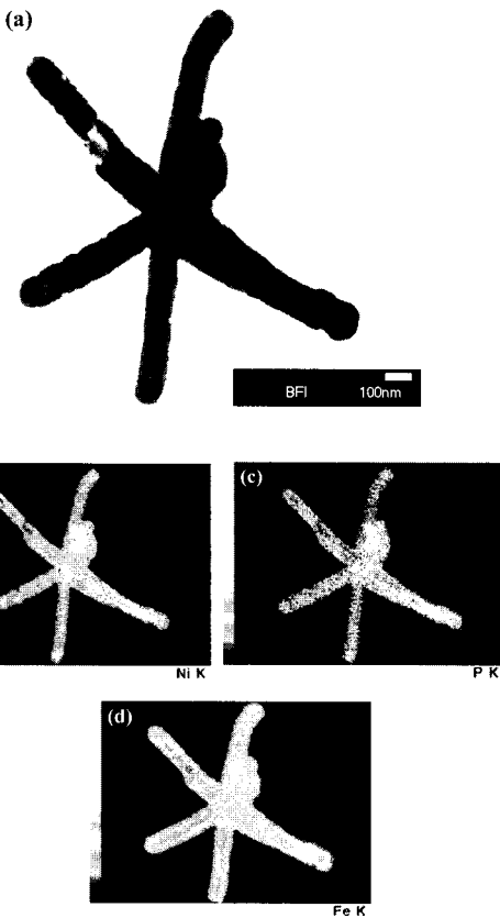
Fig. 8 (a) TEM BF image and (b), (c), (d) EDS map for Ni, P, Fe elements of Ni-Fe coated CNFs.
