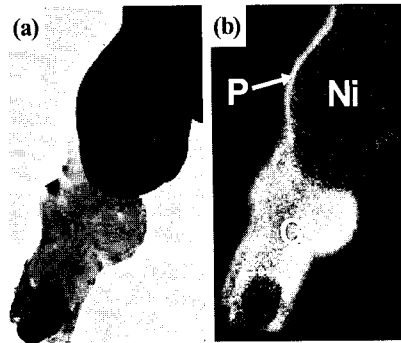
Fig. 4 (a) TEM BF image and (b) EELS map for C, Ni, P elements of Ni-P coated CNFs with uncoated layers.
