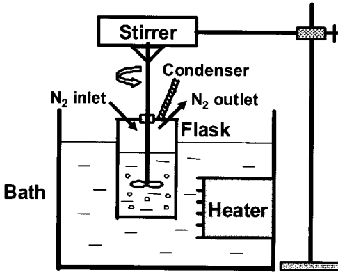
Fig. 2 Experiment setup for electroless plating.
