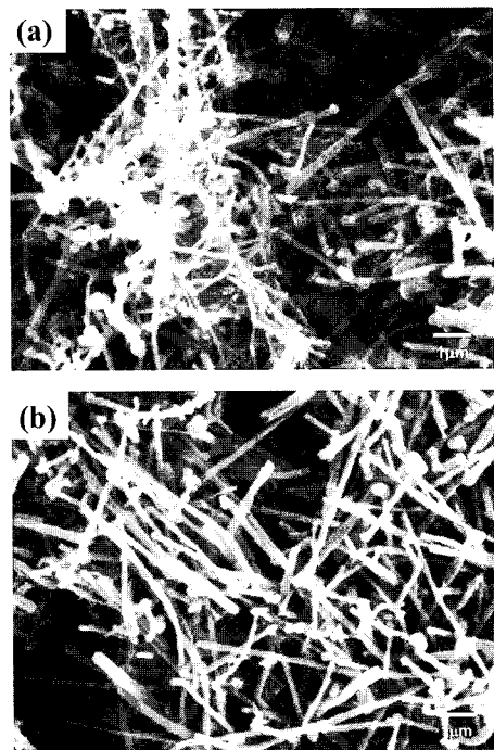
Fig. 1 SEM images of (a) as-received CNFs (b) pre-treated CNFs.
