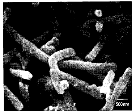
Fig. 5 SEM image of as-fabricated Ni-P coated CNFs.
