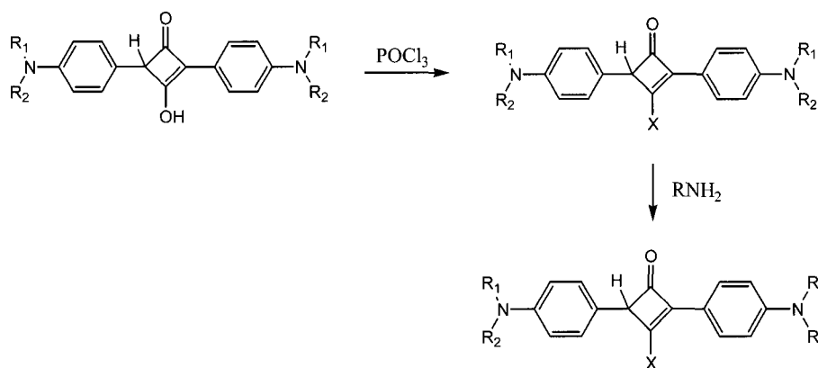
Scheme 3. The synthesis route of leuco amino-squarylium.
