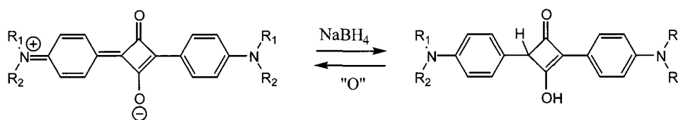
Scheme 2. Formation of leuco 1,3-squaraines.
