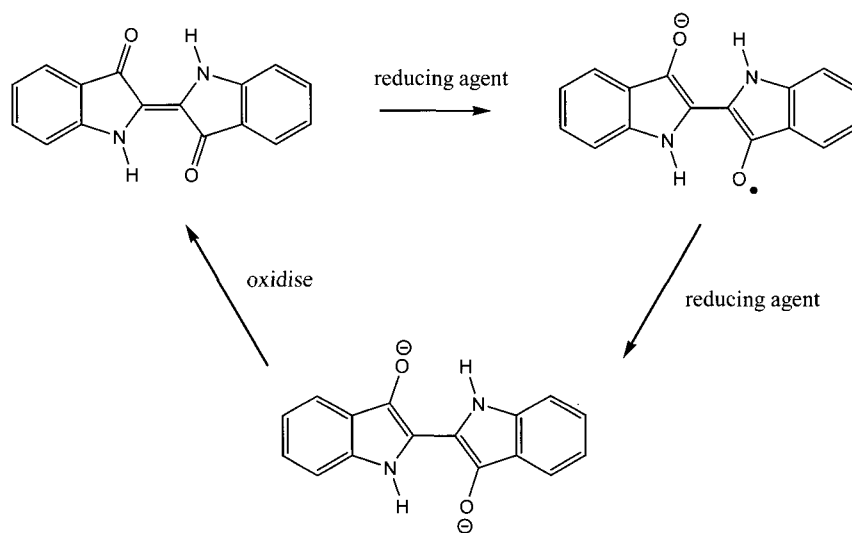
leuco dianion Scheme 1. Oxidation / reduction of indigo.
