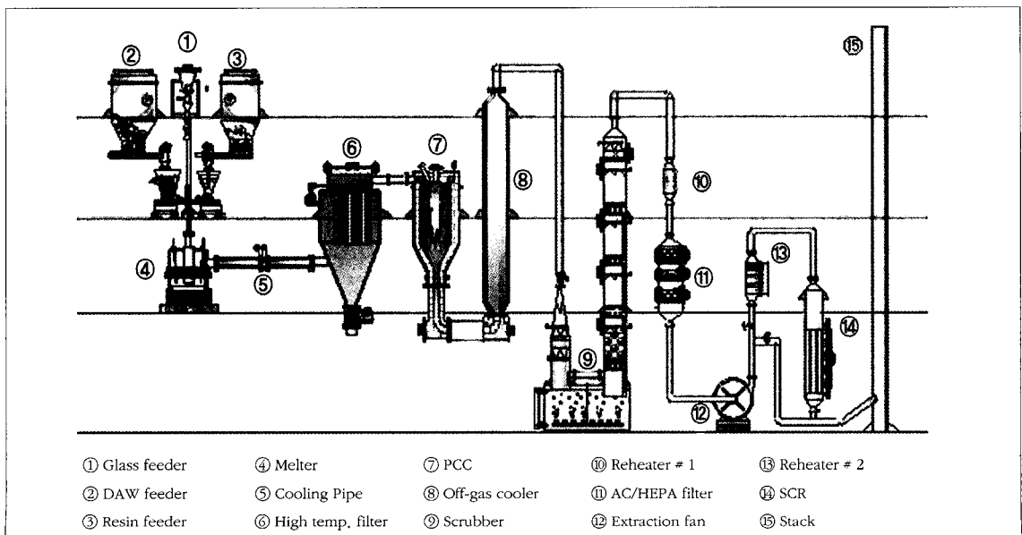
Fig. 1. Schematic of Vitrification Plant.
