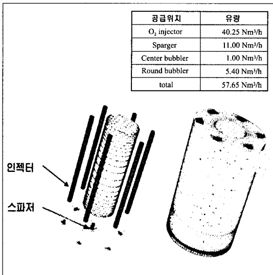
Fig. 2. Mesh for Analysis of CCM.
