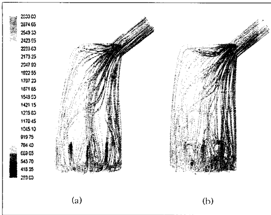
Fig. 5. Inner Path Line of CCM. (a) W1 20kg/h, (b) DAW 25kg/h)
