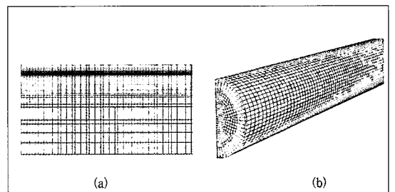
Fig. 7. Mesh for Analysis of Pipe Cooler. (a) 2D Meshed, (b) 3D Meshed.
