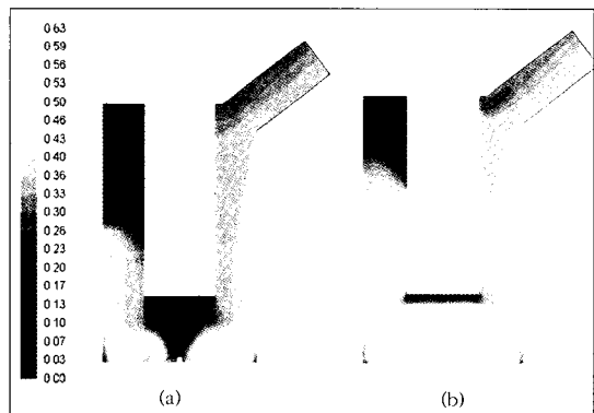
Fig. 4. Contour of CO 2 Distribution. (a) W1 20kg/h, (b) DAW 25kg/h)
