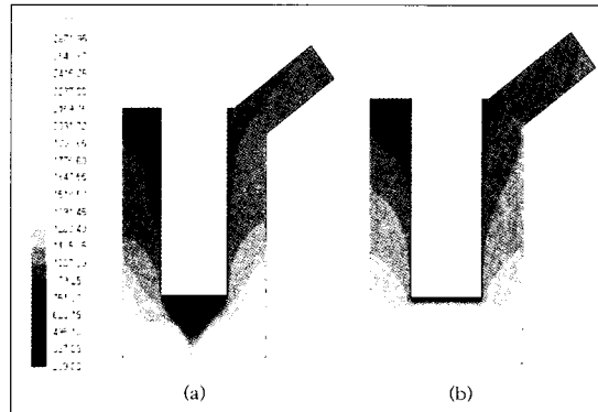
Fig. 3. Contour of Temperature. (a) W1 20kg/h, (b) DAW 25kg/h)
