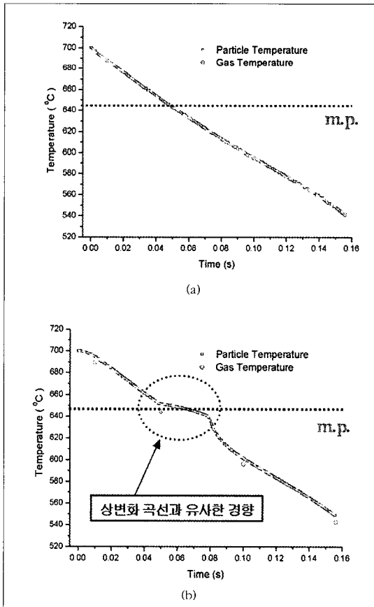
Fig. 8. Particle Temperature, Inside of Pipe Cooler. (a) Particle Diameter = 0.1 \mu m, (b) Particle Diameter = 10 \mu m
