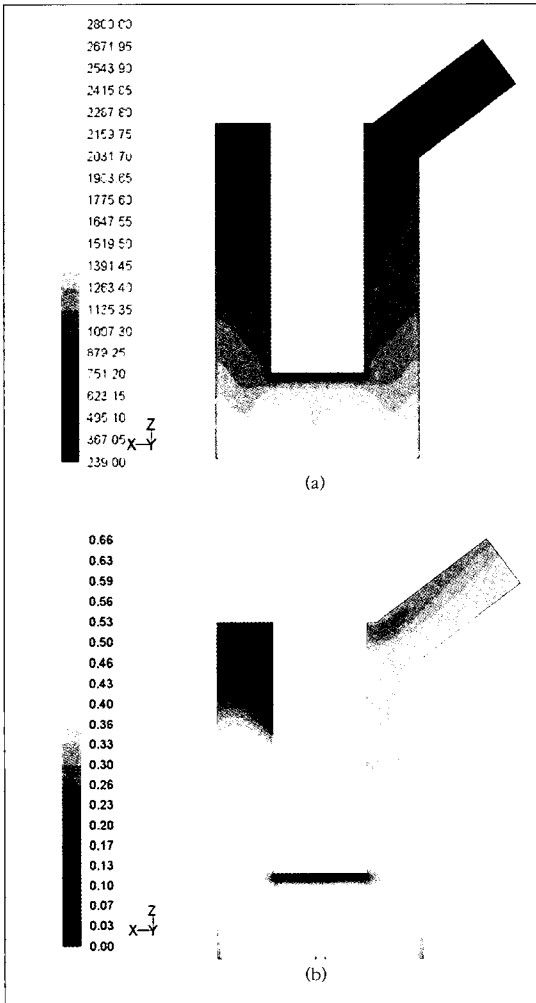
Fig. 6. Model-1 (DAW 25kg/h). (a) Contour of Temperature (b) Contour of CO 2 Distribution
