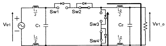
Fig. 6 Dead-time mode during forward power flow
