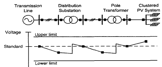
Fig. 2 Voltage curve of the clustered PV system connected with grid
