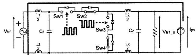
Fig. 8 Active mode during reverse power flow
