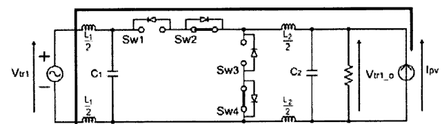
Fig. 9 Dead-time mode during reverse power flow
