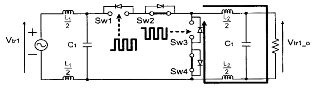
Fig. 7 Freewheeling mode during forward power flow
