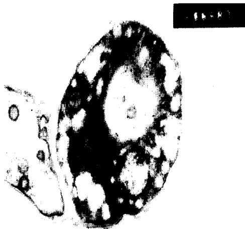
Fig. 3. G. resinaceum mycelia at 300 mM Sodium chloride (87000 ×) indicated complete cells distortion with the disappearance of cell wall layers. Cells have many vacuoles, and become to fuse with each other.
