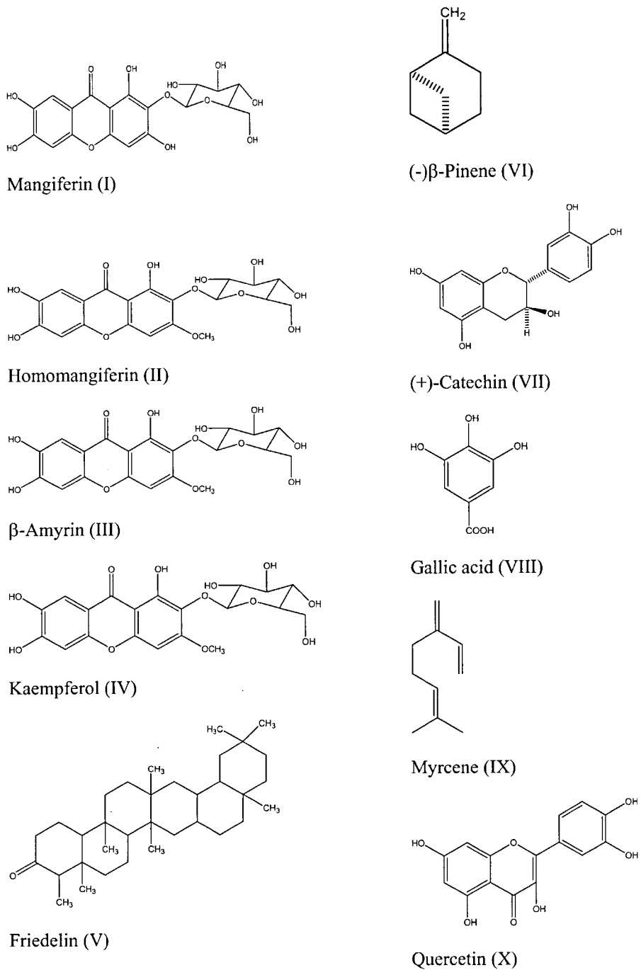
Fig. 1. Some important phytoconstituents from various parts of MI.
