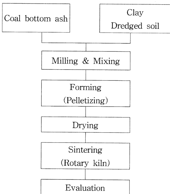
Fig. 1. Flow chart of manufacturing procedure for artificial lightweight aggregates.
