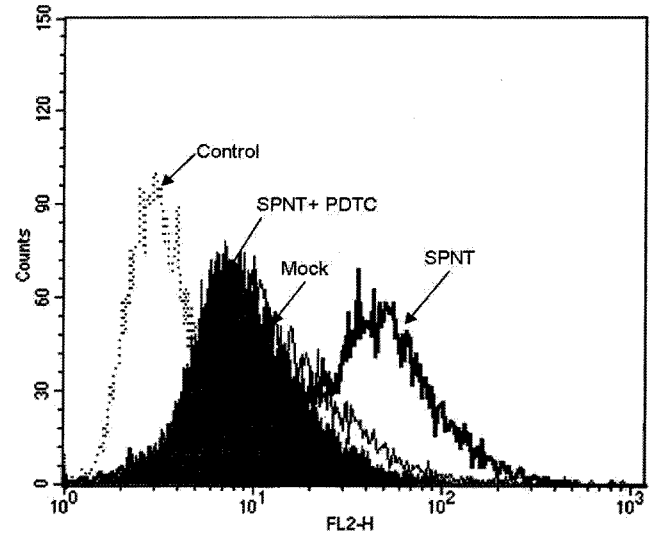
Fig. 2. Inhibition of SPNT-mediated stimulation of ICAM-1 expression by PDTC. THP-1 cells were incubated with SPNT in the presence or absence of NF-κB inhibitor PDTC (1 μM). Twenty four hr later cells were harvested and stained with PE-conjugated anti-ICAM-1 antibody and determined by flow cytometry. SPNT, supernatant obtained from HCMV-infected cells (M.O.I.=1) at 24 hr postinfection.
