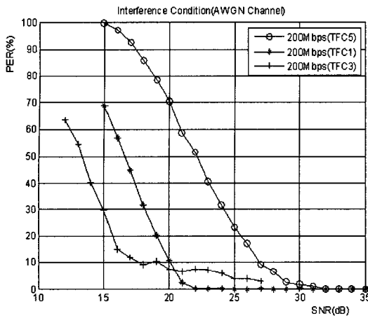
(a) AWGN 채널 환경 (a) AWGN channel environment
