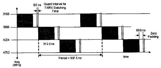
(a) TFI 모드(TFC 1) (a) TFI mode(TFC 1)
