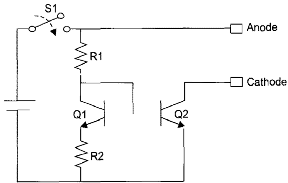
Fig 1. Schematic diagram of the electric circuit. S1, switch; Q1, Q2, transistor; R1, R2, resistor.
