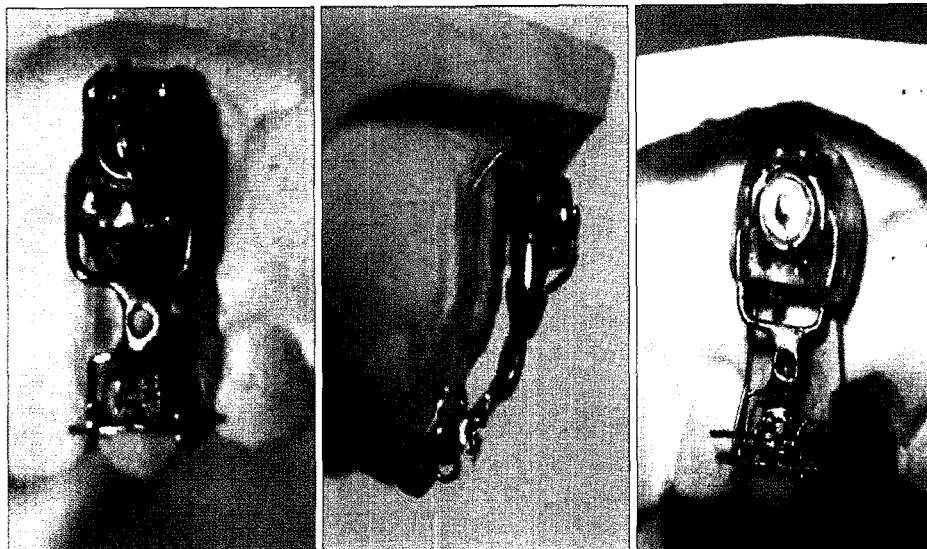
Fig 3. Assemblies, customized bracket and electric elements used in fixed electric devices.
