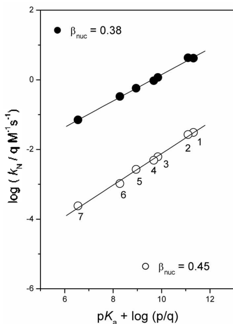
Figure 3. Brønsted-type plots for reactions of 2,4-dinitrophenyl diphenylphosphinate 3 (●) and 4-nitrophenyl diphenylphosphinate 4 (○) with alicyclic secondary amines in 80 mol % H 2 O/20 mol % DMSO at 25.0 ± 0.1 °C. The identity of the points is given in Table 1.
