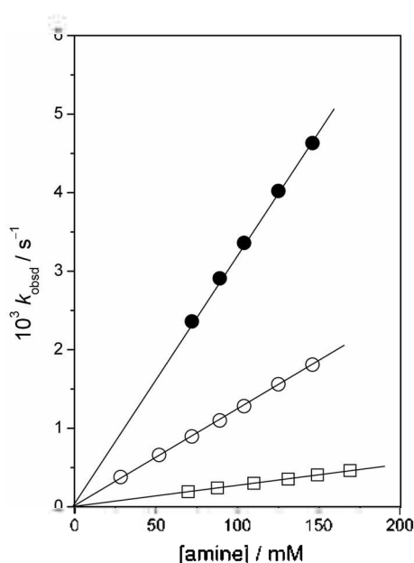
Figure 1. Plots of k_{\text{obsd}} vs. [amine] for reactions of 4-nitrophenyl diphenylphosphinate ( 4 ) with piperidine (●), piperazine (○), and morpholine (□) in 80 mol % H 2 O/20 mol % DMSO at 25.0 ± 0.1 °C.
