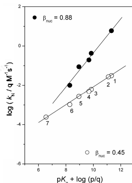
Figure 2. Brønsted-type plots for the reactions of 4-nitrophenyl benzoate 2 (●) and 4-nitrophenyl diphenylphosphinate 4 (○) with alicyclic secondary amines in 80 mol % H 2 O/20 mol % DMSO at 25.0 ± 0.1 °C. The identity of the points is given in Table 1.
