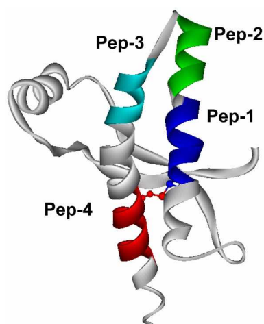
Figure 1. NMR structure 39 of the human PrP C residues 121-231. The peptide segments of PrP C used for generating the IgY Ab-s are: residues 179-186 (Pep-1), 189-195 (Pep-2), 199-205 (Pep-3) and 214-221 (Pep-4). The disulfide bond between the helices is indicated.
