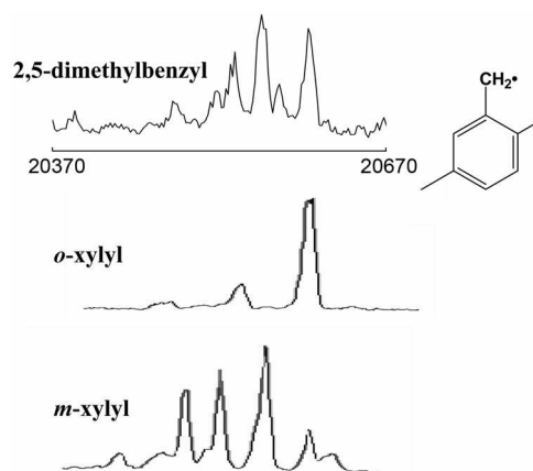
Figure 6. Comparison of band shape of origin band of 2,5-dimethylbenzyl radical with those of o - and m -xylyl radicals.
