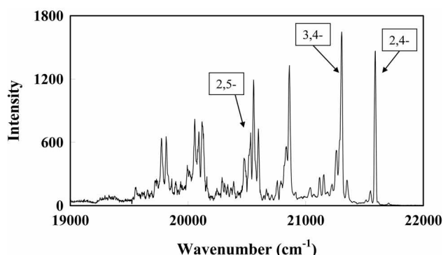
Figure 1. Vibronic emission spectrum observed from precursor 1,2,4-trimethylbenzyl radicals with a large amount of inert carrier gas helium in CESE.
