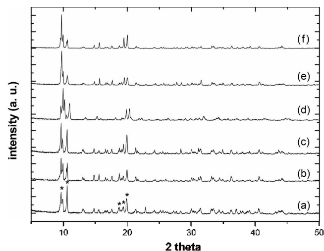
Figure 9. XRPD patterns of polymers: (a) an original form (polymer 1·dmf ); (b) a guest-free form (polymer 1 ); (c) a dmf-resorbed form (polymer 1 ); (d) a CH 3 CN-resorbed form (polymer 1·CH 3 CN ); (e) an acetone-resorbed form (polymer 1·acetone ); (f) a thf-resorbed form (polymer 1·thf ).
