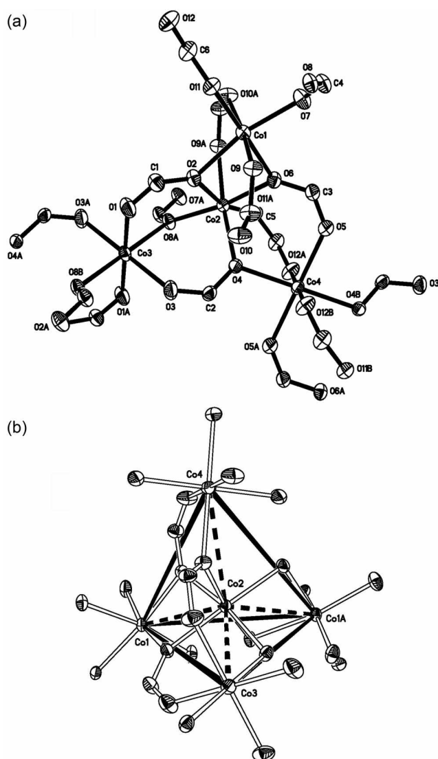
Figure 1. (a) Local coordination environments of Co metals in polymer 1-dmf . (b) The distorted tetrahedral Co 4 node with Co 2 at its center.
