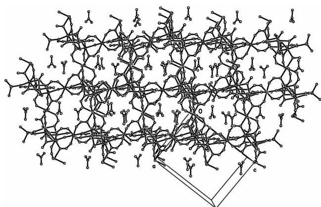
Figure 7. Packing diagram of polymer 1·acetone along the b -axis.
