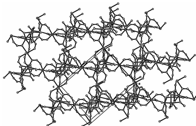
Figure 5. Packing diagram of polymer 1 along the b -axis.
