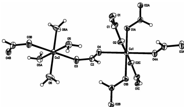
Figure 3. Local coordination environments of Co metals in polymer 2 .
