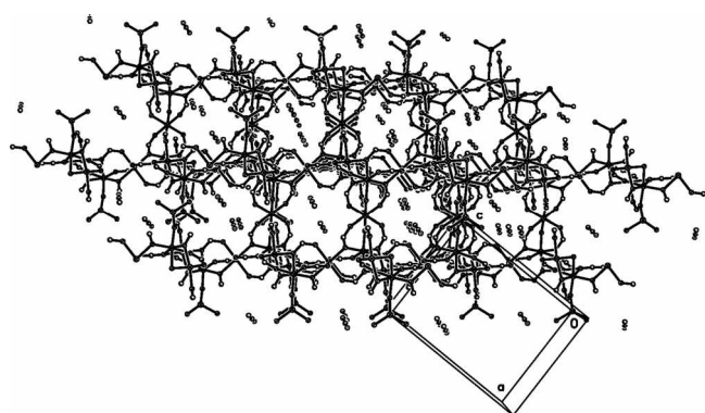
Figure 6. Packing diagram of polymer 1·CH 3 CN along the b -axis.
