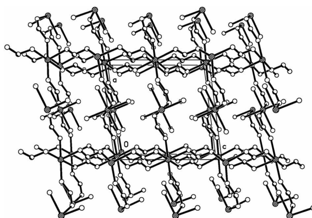
Figure 4. A packing diagram of polymer 2 along the b -axis.
