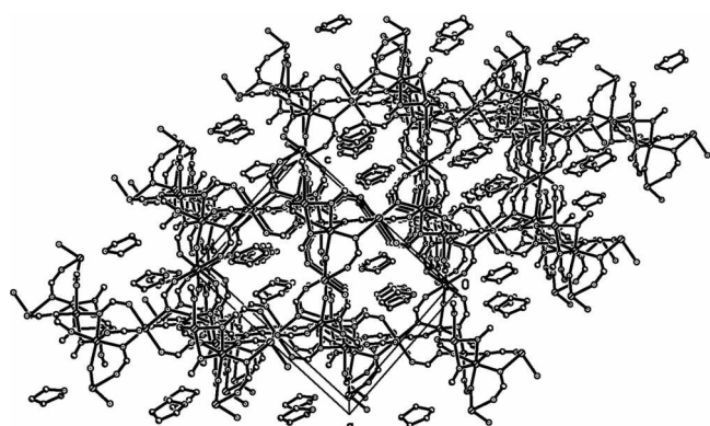
Figure 8. Packing diagram of polymer 1·thf along the b -axis.
