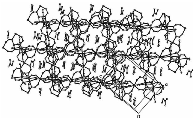
Figure 2. Packing diagram of polymer 1·dmf along the b -axis.
