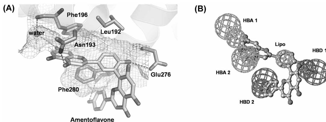
Figure 2. (A) Docking model of PTP1B and amentoflavone. Side chain of Phe196, Leu192, and Phe280 participated in hydrophobic interactions with amentoflavone. (B) Optimal pharmacophore map, Map 3.
