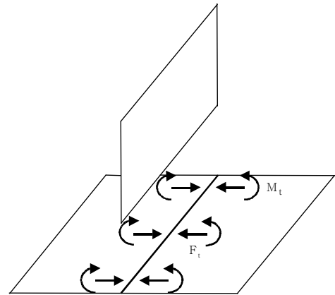
Fig. 1 Simplified model of fillet welding process
