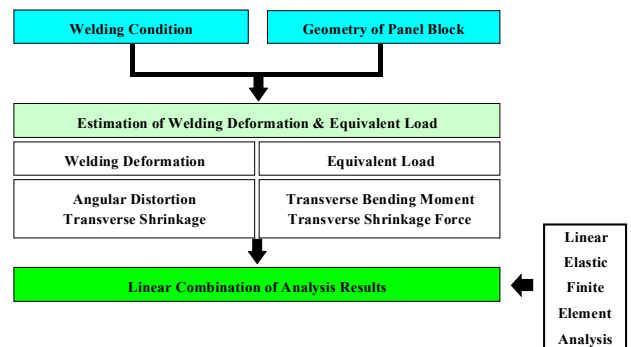
Fig. 2 Simplified analysis procedure for the prediction of welding deformation
