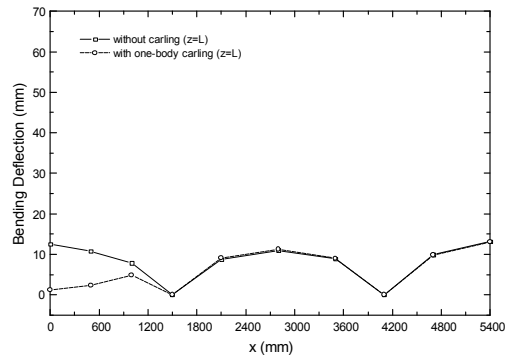
(a) Longitudinal deformation
