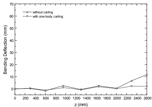
(b) Transverse deformation
