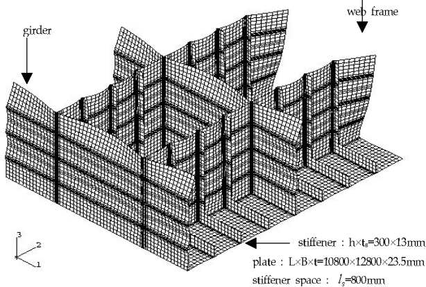
Fig. 7 Simulation result for tank top block model without carling at sub-assembly stage
