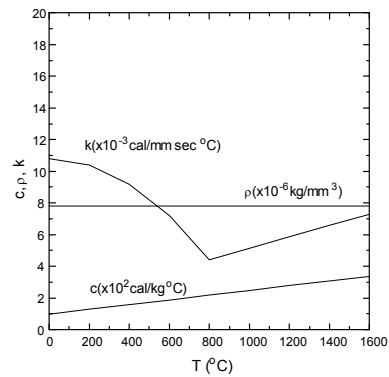
Fig. 4 Temperature-dependent physical properties of AH32 high tensile steel
