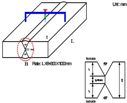
Fig. 1 Dimension of experimental model
