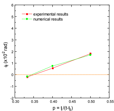
Fig. 11 Comparison of numerical results with measured results
