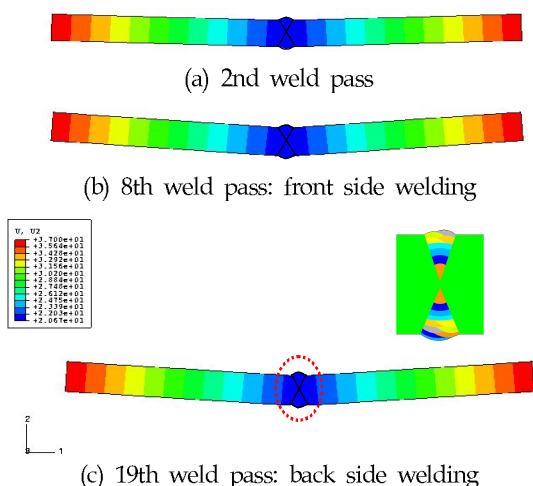
Fig. 9 Deformed shape due to X-groove butt welding for Model-X1
