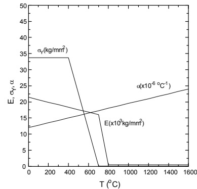
Fig. 5 Temperature-dependent mechanical properties of AH32 high tensile steel
