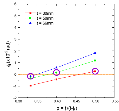
Fig. 3 Most suitable groove shape to minimize the angular distortion
