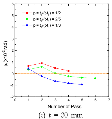
Fig. 2 Influence of pass number on the angular distortion
