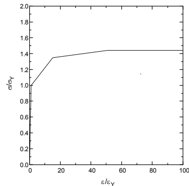
Fig. 6 Strain hardening model for AH32 high tensile steel
