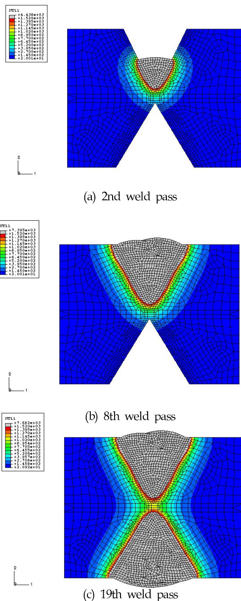
Fig. 7 Temperature history for Model-X1 varying with weld pass
