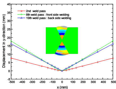
Fig. 10 Computed angular distortion for Model-X1
