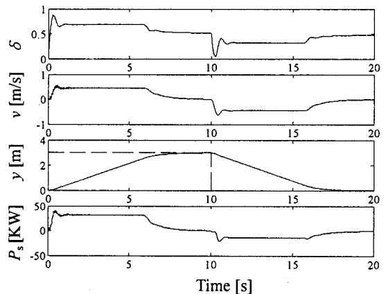
Fig. 8 Simulation result 1 (circuit1, p_s=20\text{MPa} , H=3\text{m} , \gamma=0.5 )
