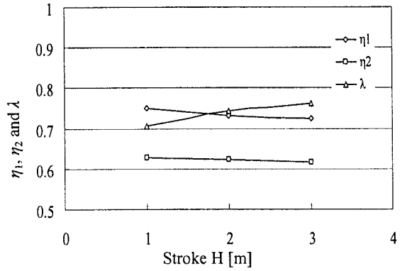
Fig. 12 Influence of supply pressure (circuit 1, H=1\text{m} , \gamma=0.5 )
