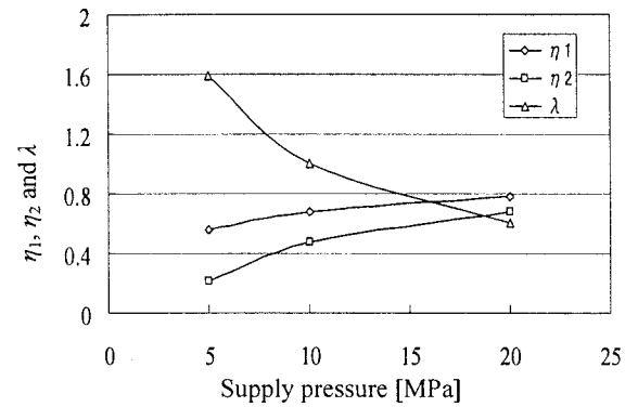
Fig. 14 Influence of stroke (circuit 1, p_s=20\text{MPa} , \gamma=0.5 )
