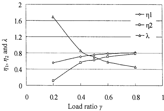
Fig. 10 Influence of load ratio (circuit 1, p_s=20\text{MPa} , H=1\text{m} )
