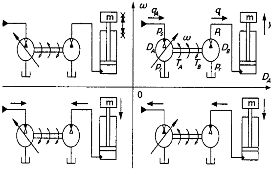
Fig. 4 Driving state of transformer and cylinder (circuit1)
