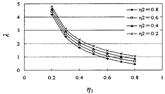
Fig. 7 Relation between efficiency and energy
