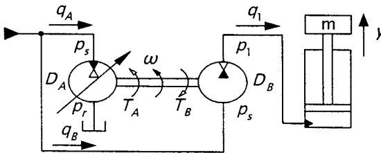
Fig. 2 Hydraulic circuit 2
