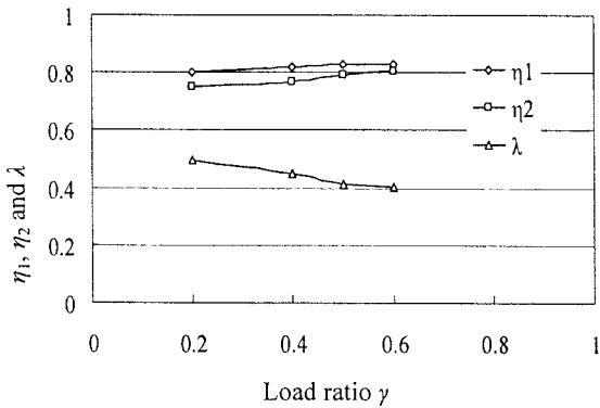
Fig. 11 Influence of load ratio (circuit 2, p_s=10\text{MPa} , H=1\text{m} )
