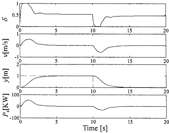
Fig. 9 Simulation result 2 (circuit2, p_s=10\text{MPa} , H=1\text{m} , \gamma=0.5 )
