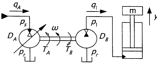
Fig. 1 Hydraulic circuit 1
