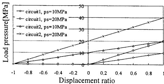
Fig. 3 Relation of displacement and load pressure
