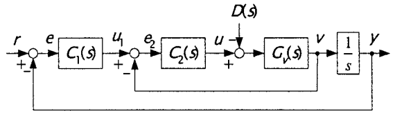
Fig. 6 Cylinder position control system
