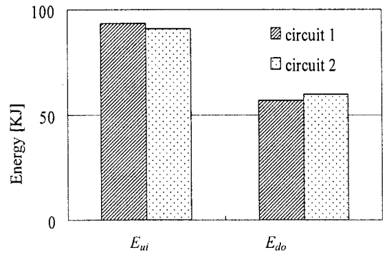
Fig. 13 Energy consumption for different solution (circuit1: H=1\text{m} , m=7692\text{kg} , \gamma=0.75 , p_s=20\text{MPa} circuit2: H=1\text{m} , m=7692\text{kg} , \gamma=0.5 , p_s=10\text{MPa} )
