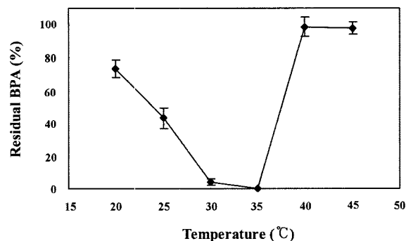
Fig. 2. Degradation of 50 mg/L bisphenol A (BPA) by T. versicolor in 12 hr at different temperature when the fungal inocula were added with BPA into YMG medium.
