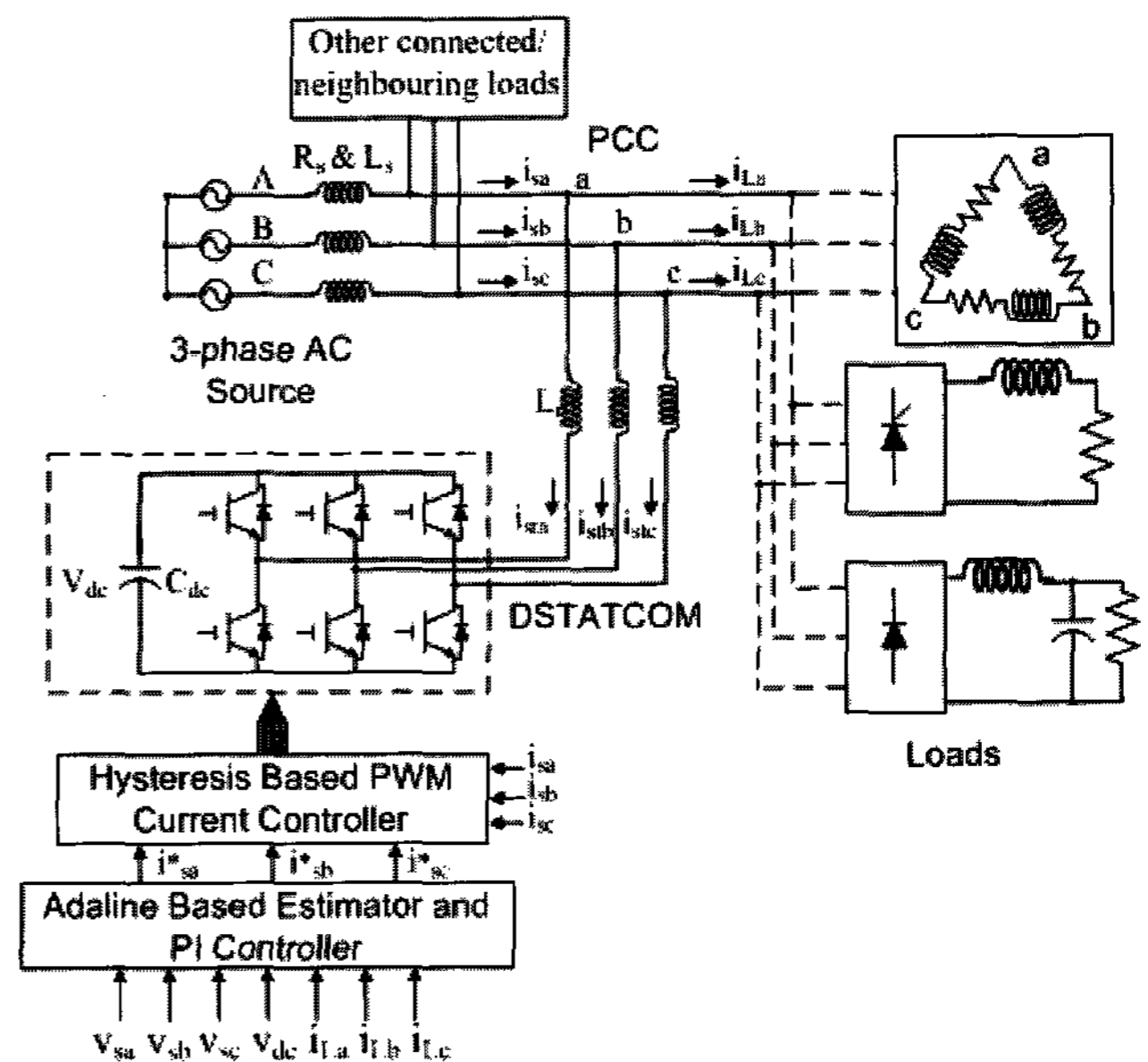
Fig. 1 Basic circuit diagram of the DSTATCOM system
