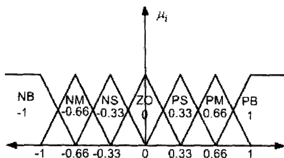
Fig. 4 Membership function for linguistic variables of L
