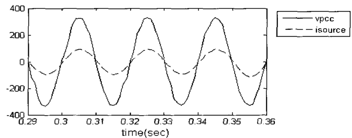
Fig. 10 Source current I_{sa} and voltage v_{sa} vs. time
