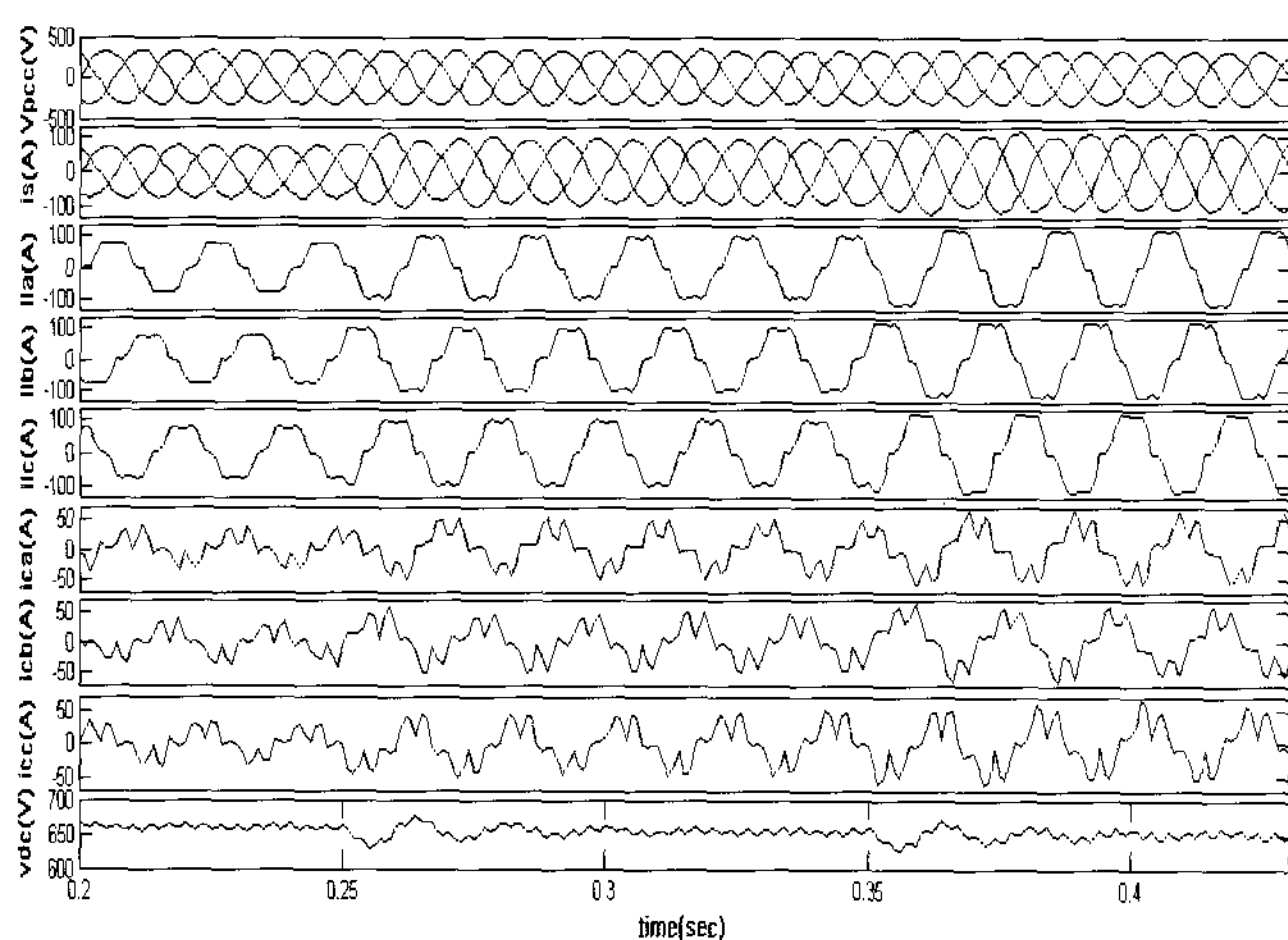
Fig. 6 Transient Performance of the system for simple PI controller for load changes from 10\Omega to 6\Omega and then to 5.12\Omega at 0.25 sec and 0.35 sec respectively
