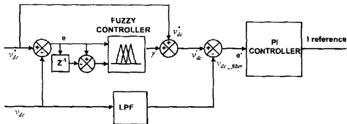
Fig. 3 Basic control scheme of fuzzy pre-compensated controller
