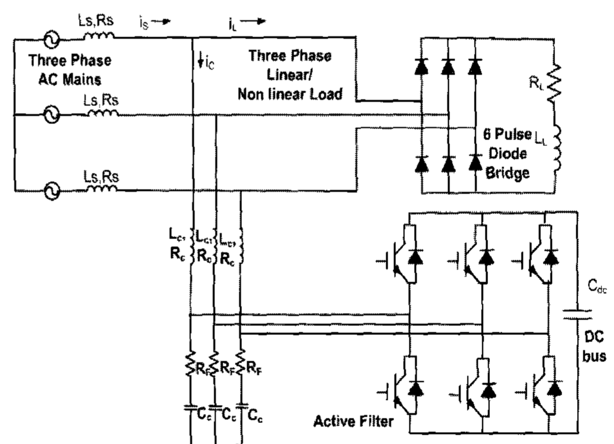
Fig. 1 Fundamental building block of active filter
