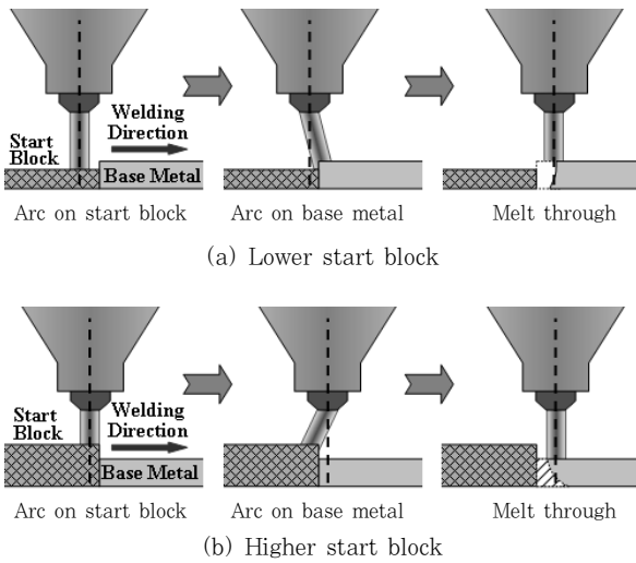
Fig. 5 Schematic diagrams of arc eccentricity with start block height
