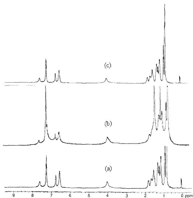
Figure 1. ^1\text{H-NMR} spectra of (a) poly[( \text{OC}_{10} ) _2 -spirobifluorene], (b) poly[( \text{OC}_{10} ) _2 -spirobifluorene-TPA] (5:1), and (c) poly[( \text{OC}_{10} ) _2 -spirobifluorene-TPA] (9:1).
