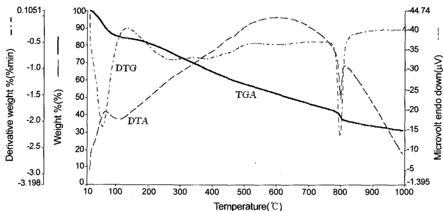
Figure 4. TGA-DTG-DTA curves of O-2-PMAP-Co complexes.
