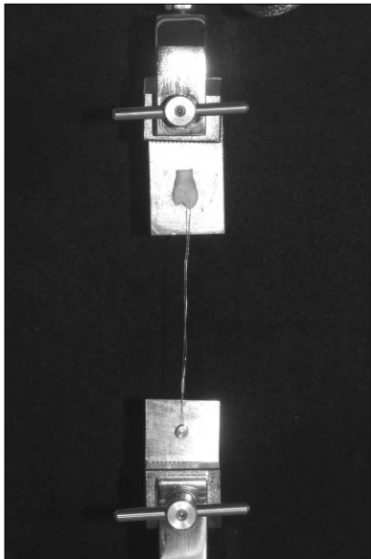
Figure 1. Microshear bond test of specimen.
