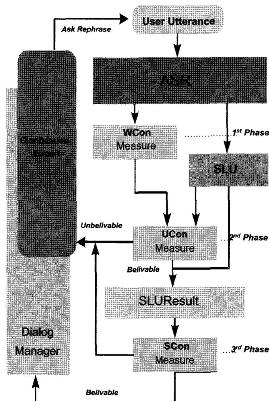
Fig. 6. Flow of error verification and clarification.
