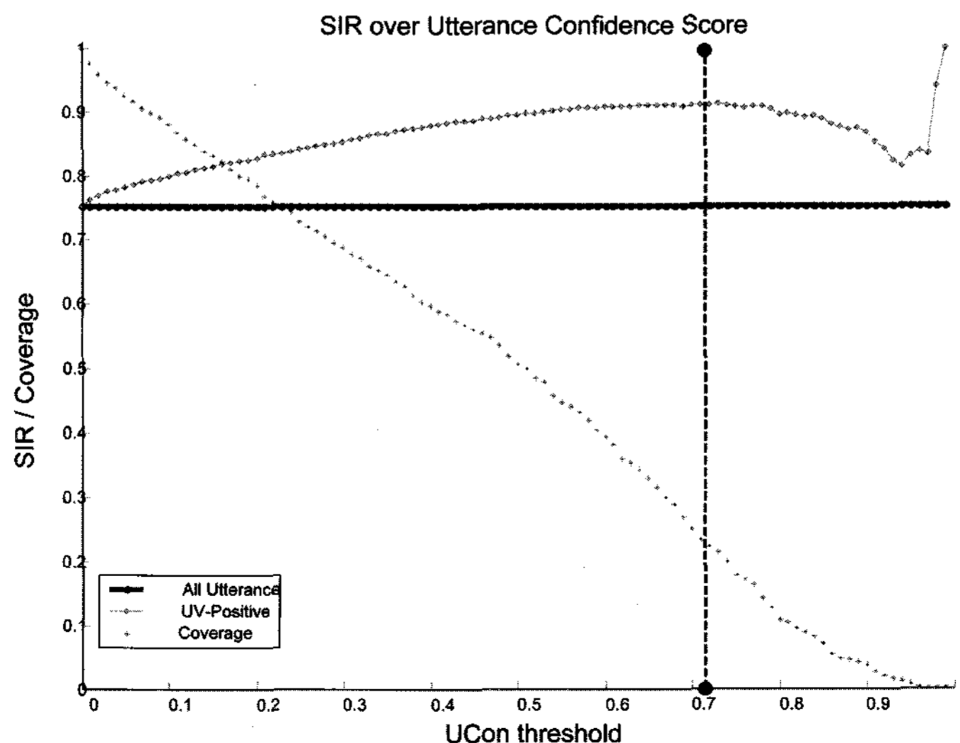
Fig. 10. SIR vs. UCon Threshold.
