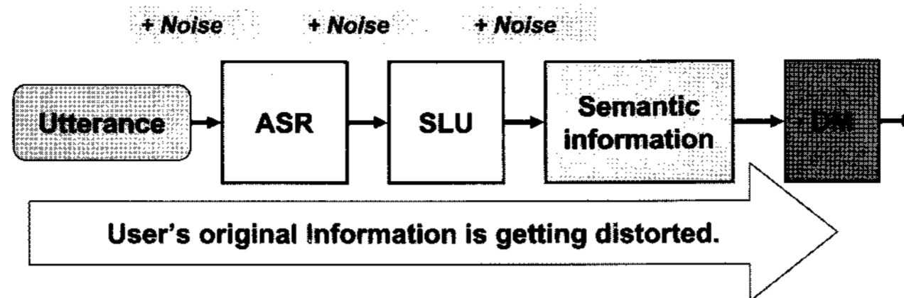
Fig. 3. Typical dialog process.
