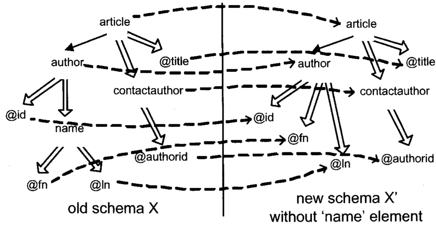
Fig. 14. Capturing the evolution of an XML schema.
