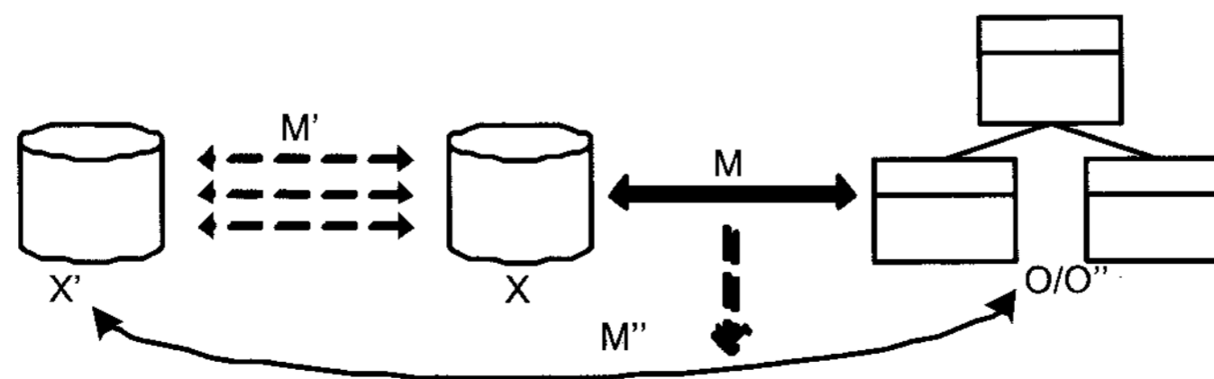
Fig. 15. Maintenance of semantic mapping.
