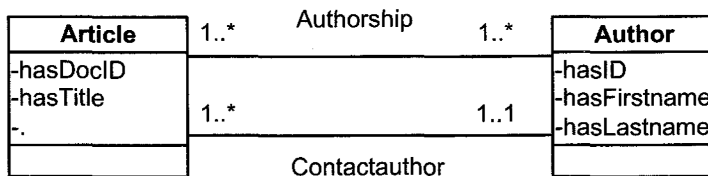
Fig. 3. An ontology.
