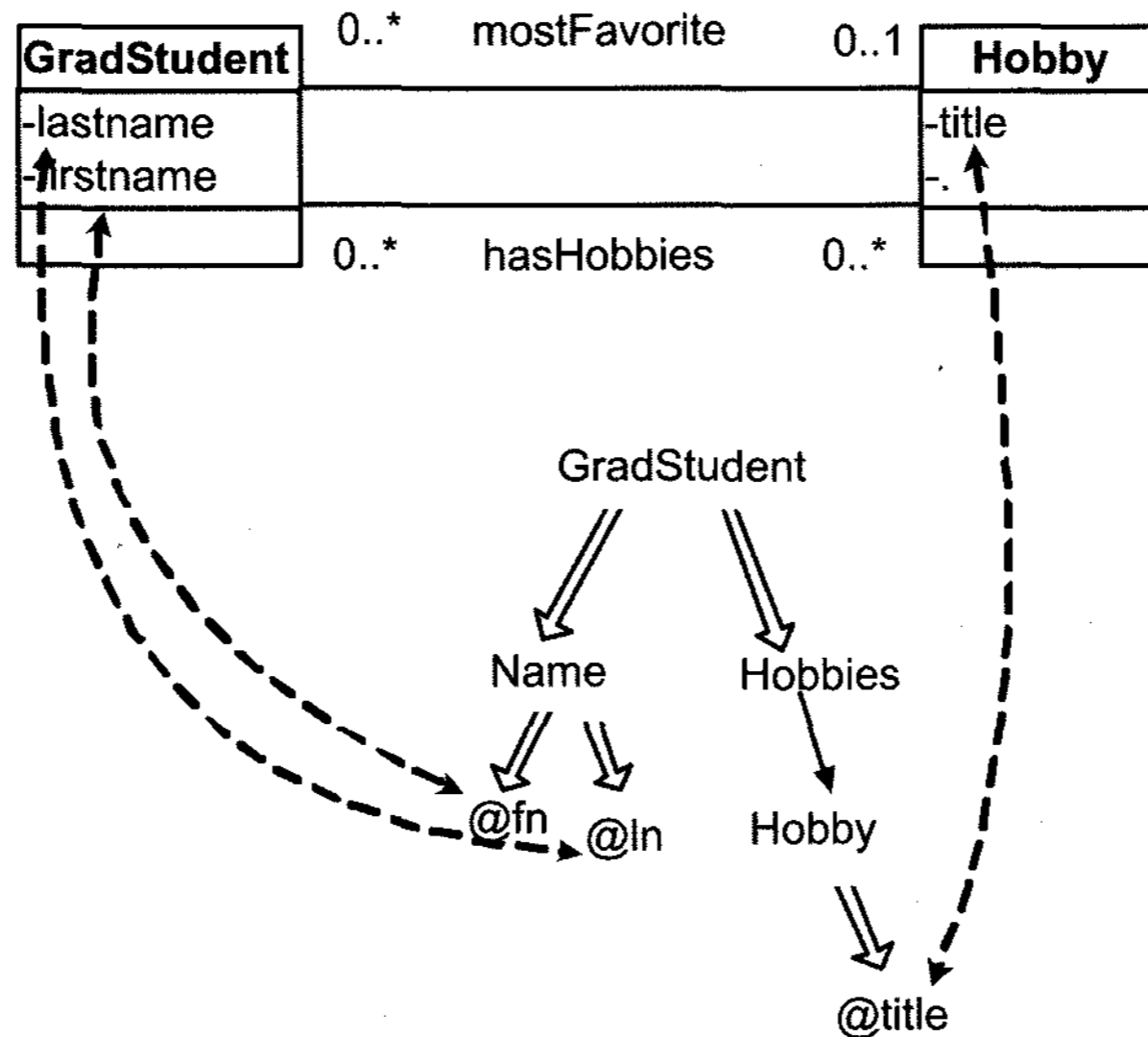
Fig. 11. An element tree with a collection tag.
