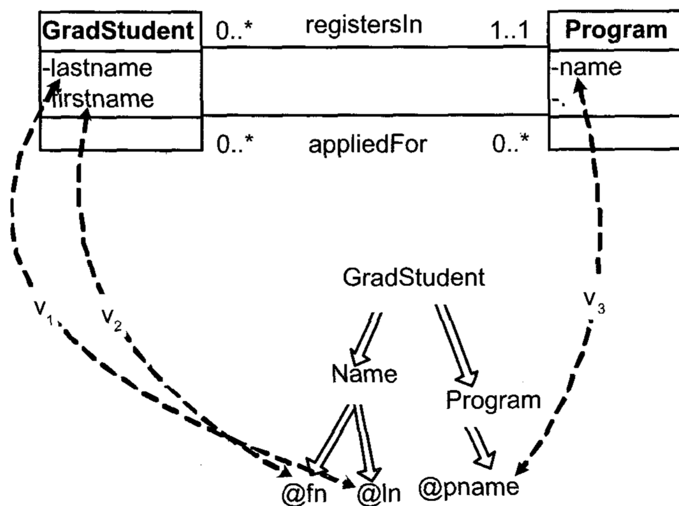
Fig. 10. An element tree and an ontology.
