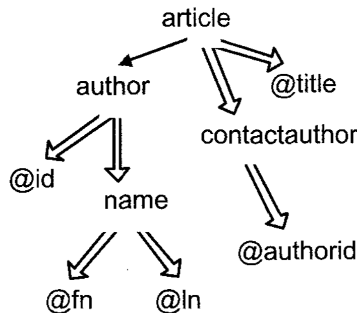
Fig. 4. An XML schema graph.
