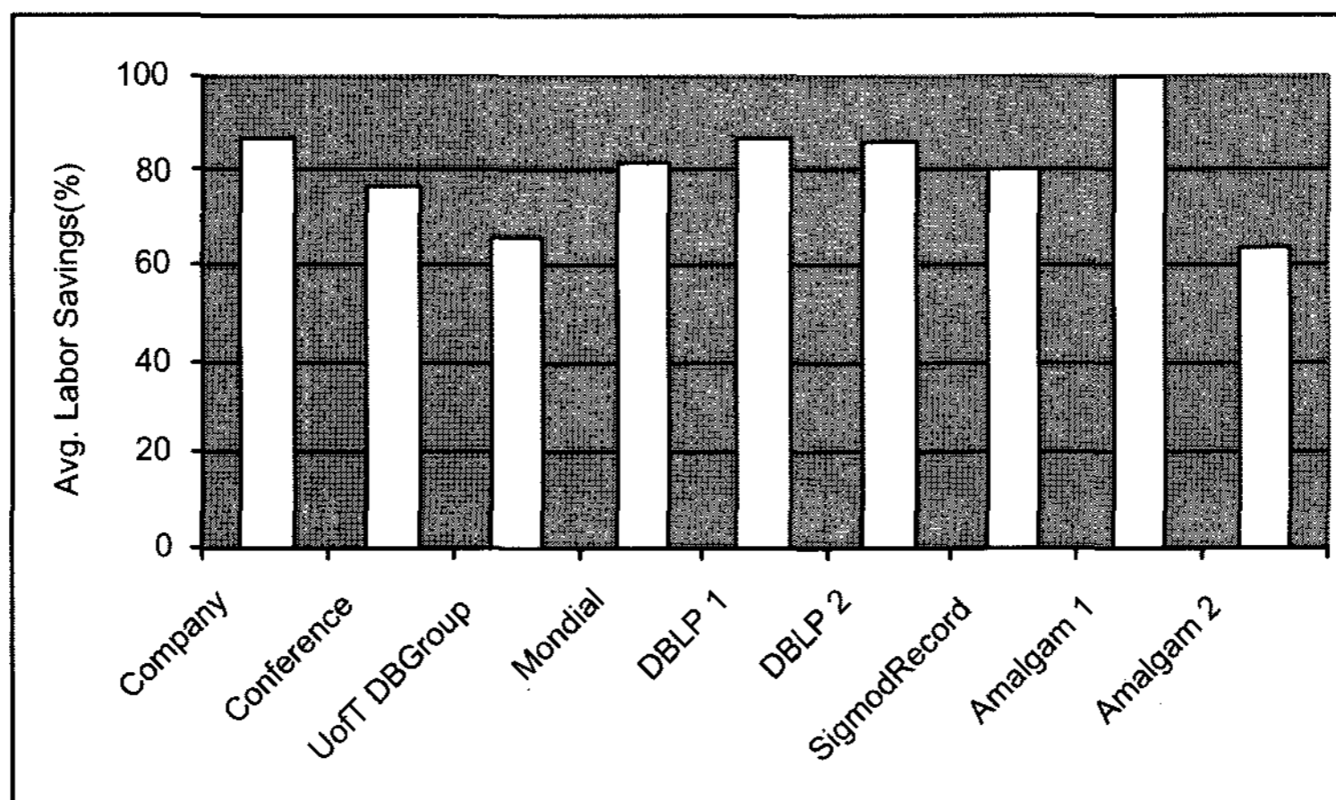
Fig. 13. Average labor savings for 9 mapping cases.
