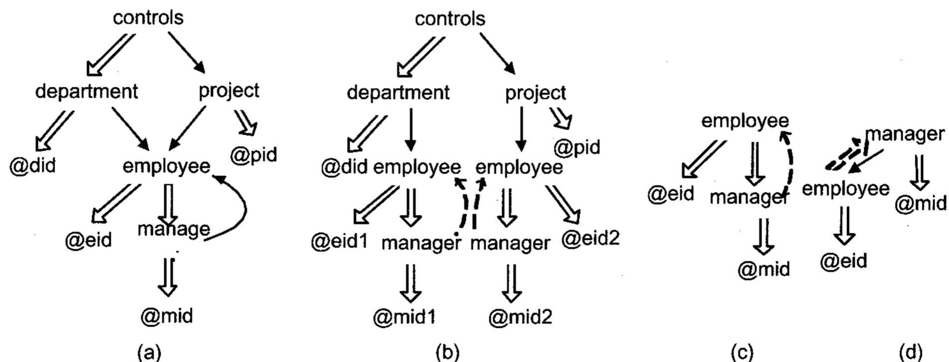
Fig. 5. Schema graph and element graphs.
