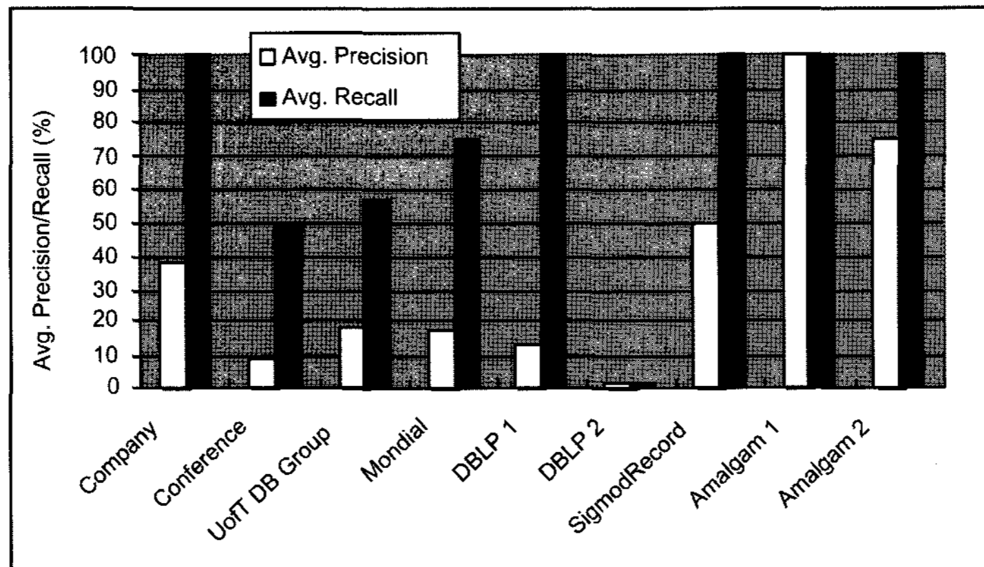
Fig. 12. Average recall and precision for 9 mapping cases.
