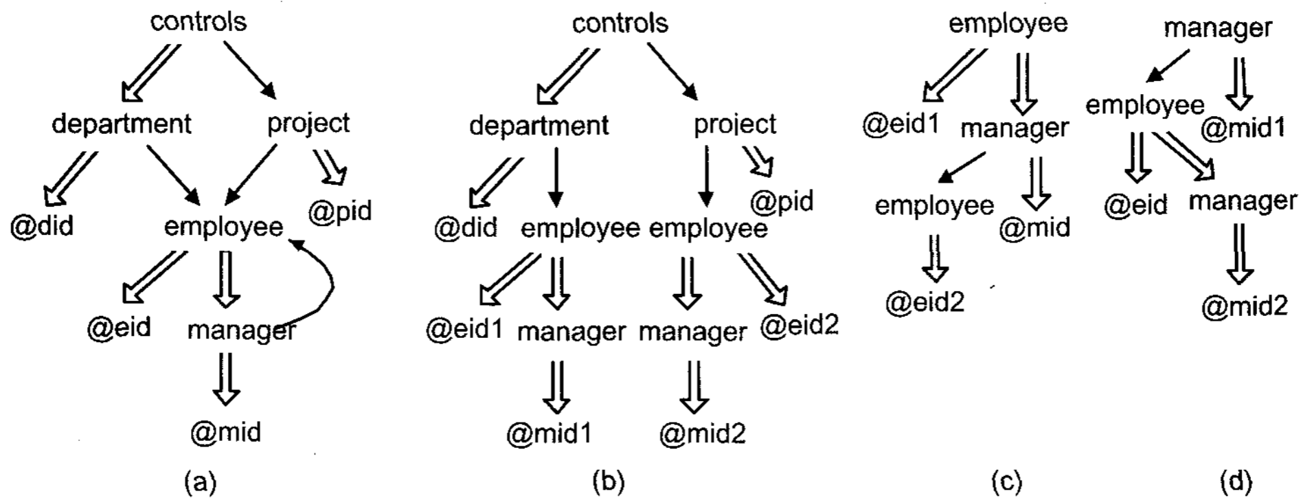
Fig. 6. Schema graph and element trees.
