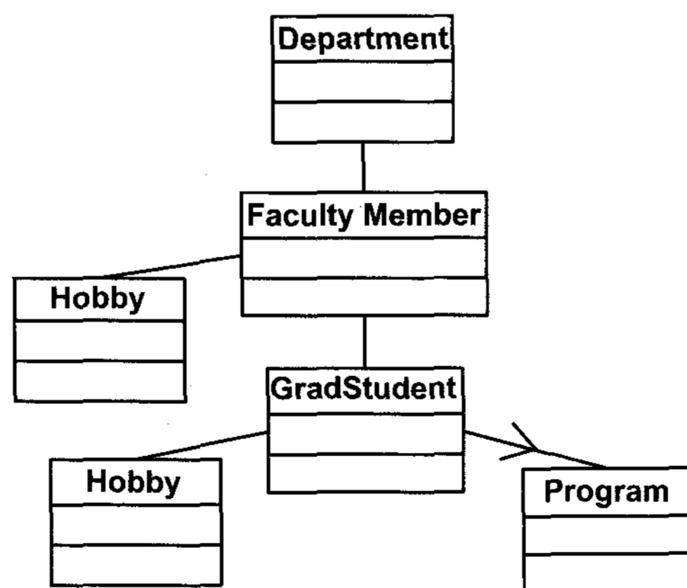
Fig. 8. The identified semantic tree.
