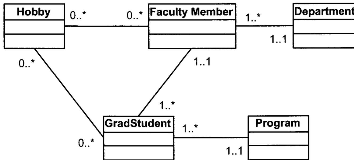
Fig. 7. A Sample CM graph.
