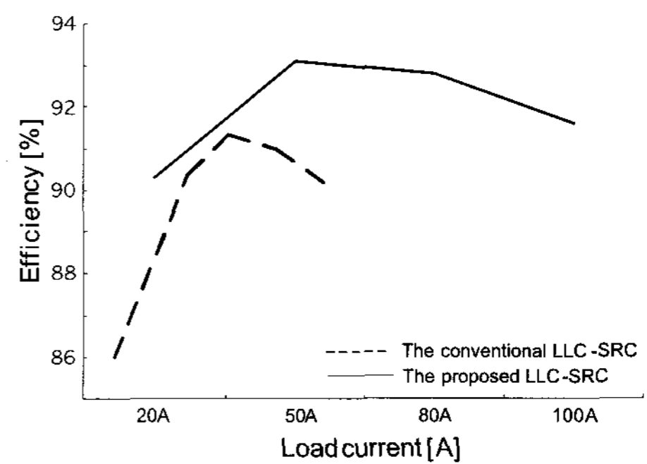
Fig. 5 Efficiency with load variation
