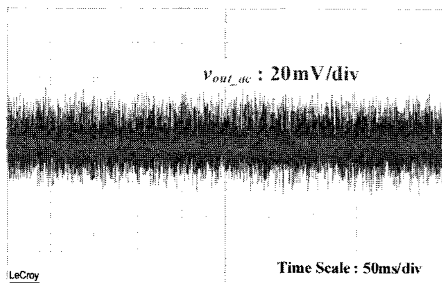
Fig. 4 The waveform of the ripple output voltage
