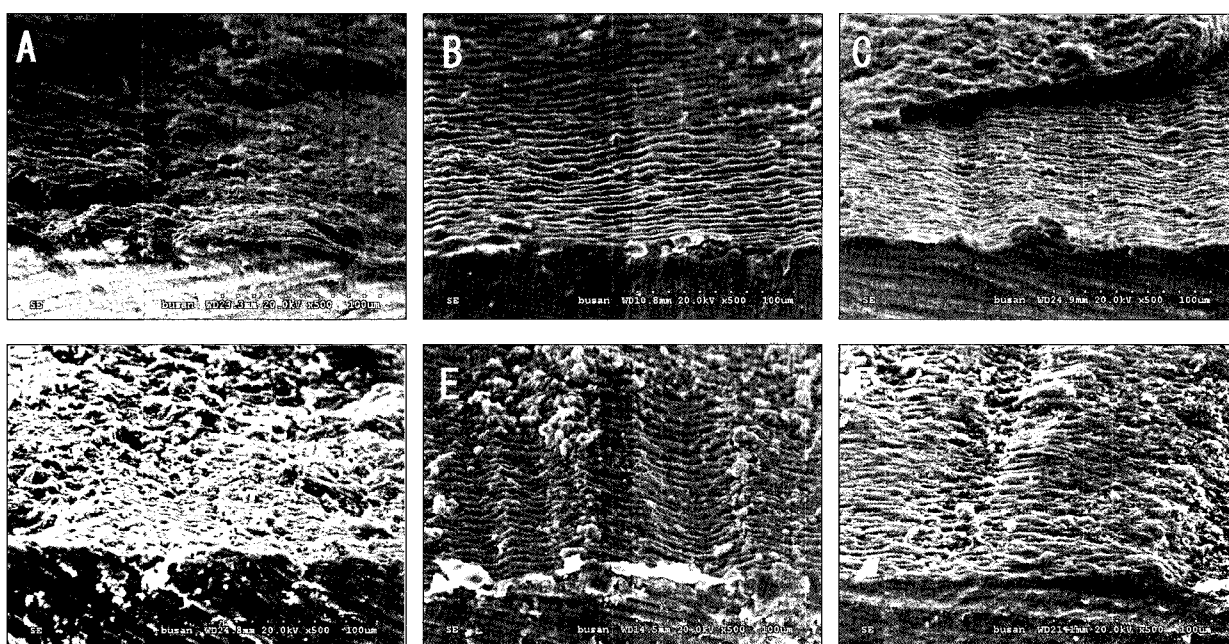
Figure 3. Representatives of SEM examination of failure surfaces of A: GMC, B: GME, C: GVL, D: RMC, E: RME, and F: RVL.
