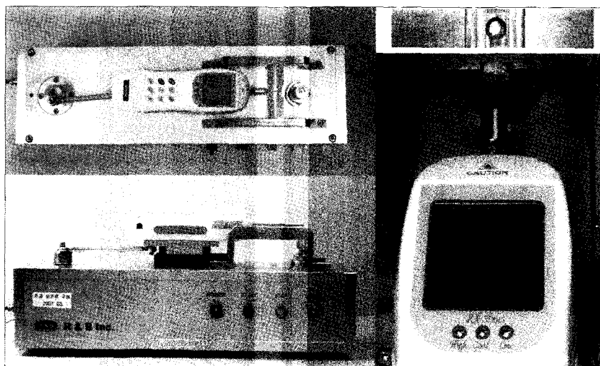
Figure 2. Push-out bond strength measuring device.
