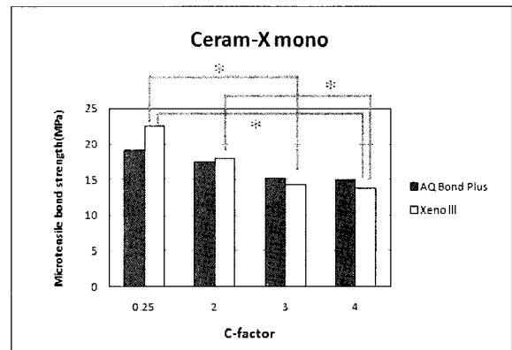
Figure 6. Graph of the mean microtensile bond strength (MPa) of the Ceram-X mono groups. Symbols (*) indicate statistical significance at p = 0.05 level
