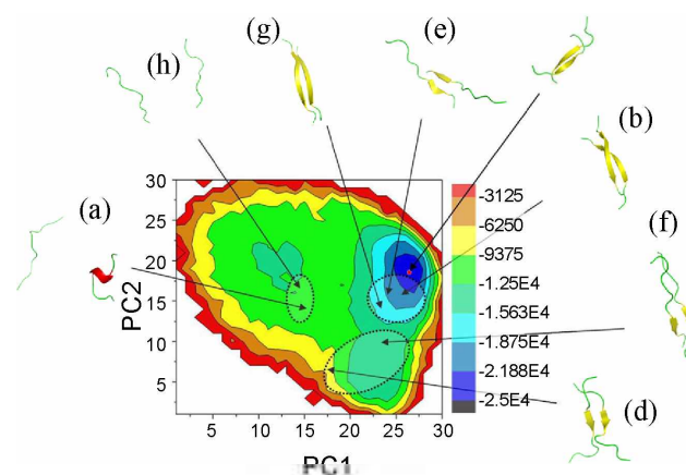
Figure 10. Free energy surface as a function of the two main principal components obtained from the trajectory of the last 120 ns for dimer simulations for residues 71–82 of \alpha -synuclein with the AMBER parm96 force field. Unit of energy shown in scaling bar is \text{J}\cdot\text{mol}^{-1} . Various conformers shown in Figure 6 are located at the corresponding positions in PC space. One of the structures in cluster (b) corresponding to the middle of global minimum region is also shown.
