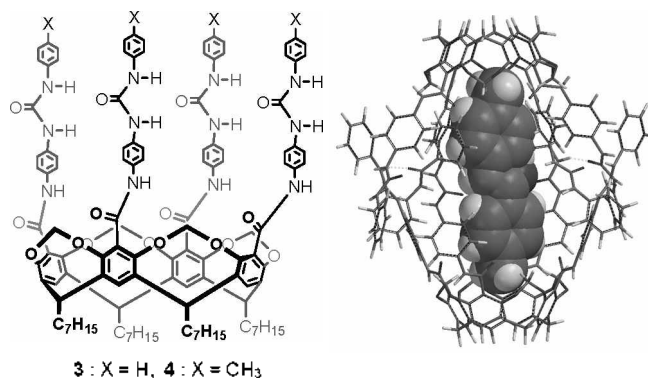
Figure 2. Ureacavitand 3 and 4, and energy minimized structure of molecular capsule 3·4-methyl- N-p -tolylbenzamide-3 by spartan'04 (MMFF Force-Field, The test were substituted by methyl for clarity).
