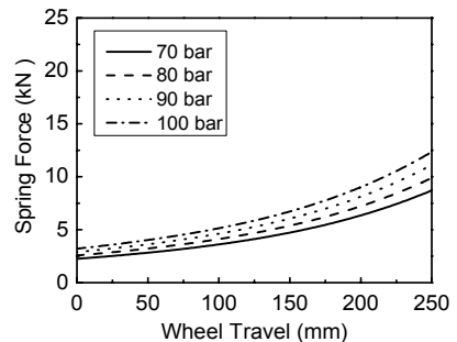
Fig. 2 Spring characteristic of MRSS
