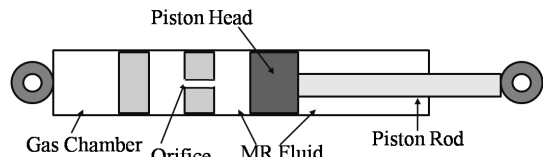
Fig. 1 Configuration of MRSS
