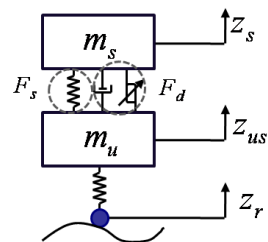
Fig. 4 Suspension system
