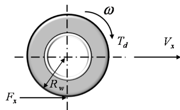
Fig. 5 Wheel rotational motion
