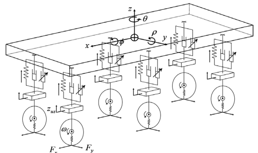
Fig. 3 Coordinate system of 6x6 vehicle
