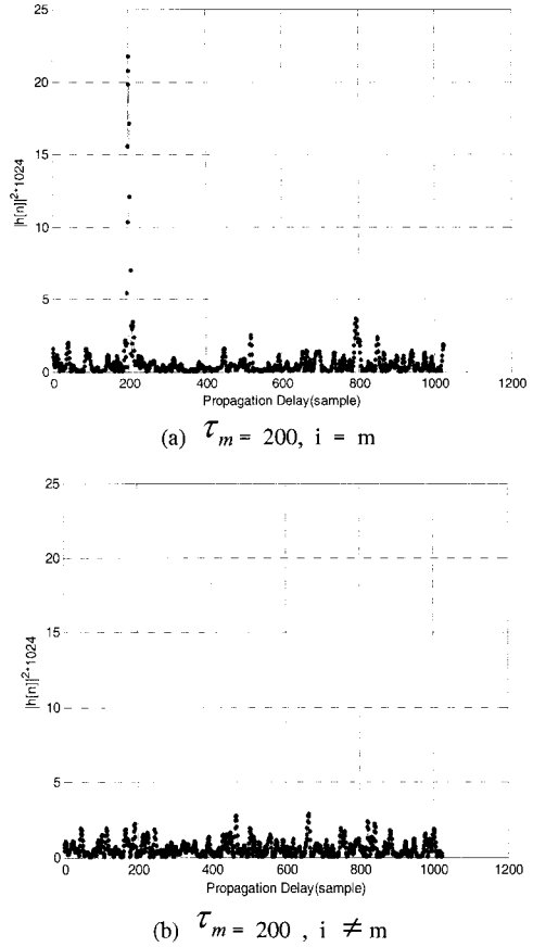
Fig. 2. Propagation Delay Estimation
