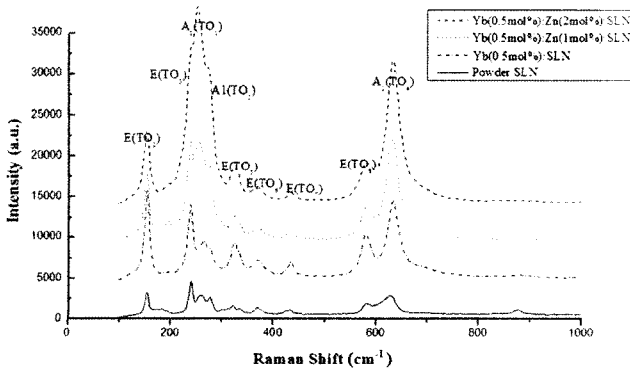
Fig. 3. Raman spectra of the Yb : Zn : LiNbO 3 rod shape single crystals.
