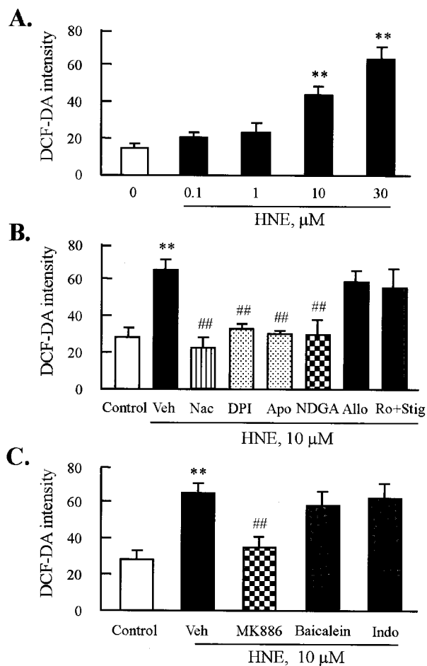
Fig. 3. Effects of inhibitors of NADPH oxidase or lipoxygenase on HNE-induced ROS production in J774A.1 macrophages. (A) Cells were treated with different concentrations of HNE for 45 min, and then ROS generation was measured by flow cytometry (FACS) using DCF fluorescence. Fluorescence intensity was analyzed by CellQuest Software. Data was presented as mean \pm SE from 5 independent experiments. ** p <0.01 vs. value at concentration 0. (B) Cells were incubated with 10 \mu M HNE for 45 min after pre-treatment with various inhibitors for ROS including N -acetylcysteine (Nac, 5 mM), diphenylamine iodonium (DPI, 10 \mu M), apocynin (Apo, 300 \mu M), nordihydroguaiaretic acid (NDGA, 10 \mu M), allopurinol (Allo, 100 \mu M), or rotenone (Ro, 1 \mu M) plus stigmatellin (Stig, 1 \mu M) for 30 min. (C) Cells were pre-treated with eicosanoid inhibitors including MK886 (10 \mu M), baicalein (10 \mu M), or indomethacin (Indo, 100 \mu M) for 30 min, and then stimulated with 10 \mu M HNE for 45 min. ROS generation was analyzed by FACS. Data was presented as mean \pm SE from 5 independent experiments. ** p <0.01 vs. control; ## p <0.01 vs. veh (vehicle).
