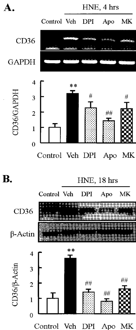
Fig. 4. Effect of inhibitors for NADPH oxidase or 5-lipoxygenase on HNE-induced CD36 expression in J774A.1 macrophages. Macrophages were treated with diphenylamine iodonium (DPI, 10 \mu M), apocynin (Apo, 300 \mu M), or MK886 (10 \mu M) for 30 min prior to HNE application. Cells were stimulated with 10 \mu M HNE for the indicated time. The levels of CD36 mRNA and protein were determined by RT-PCR (A) and Western blot analysis (B), respectively. Each fig is the representative of 5 independent experiments. Data was presented as mean \pm SE from 5 independent experiments. ** p <0.01 vs. control; # p <0.05; ## p <0.01 vs. veh (vehicle).
