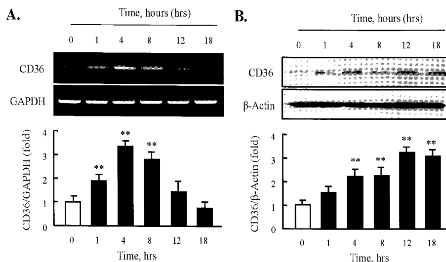
Fig. 1. Effect of HNE on the expression of CD36 in J774A.1 macrophages. (A) Total RNA was extracted from macrophages treated with 10 \mu M HNE for the indicated time (0~18 hrs). 2 \mu g RNA was subjected to RT-PCR. Band intensity for CD36 mRNA was quantified by densitometric scanning and normalized to that of GAPDH. (B) Macrophages were incubated with 10 \mu M HNE, and cellular lysates were analyzed by Western blotting using anti-CD36 antibody. \beta -actin as used to normalize density. Each photograph is the representative of 5 independent experiments. Data is presented as mean \pm SE from 5 independent experiments. ** p < 0.01 vs. value at time 0.
