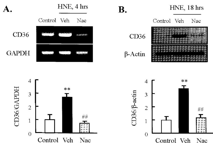
Fig. 2. Role of ROS on HNE-induced CD36 expression in J774A.1 macrophages. Macrophages were treated with 10 \mu M HNE for the indicated time in the absence or presence of N -acetylcysteine (Nac, 5 mM). The levels of CD36 mRNA and protein were determined by RT-PCR (A) and Western blot analysis (B), respectively. Each fig is the representative of 4 independent experiments. Data was presented as mean \pm SE from 5 independent experiments. ** p < 0.01 vs. control; ## p < 0.01 vs. veh (vehicle).
