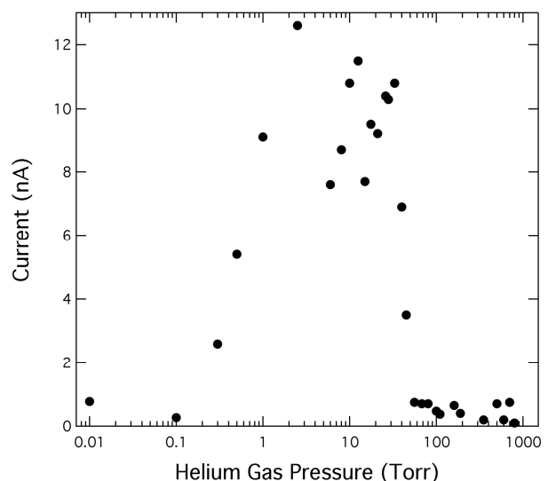
Fig. 3. The current is measured as a function of helium gas pressure. The voltage that was applied to the tungsten tip was -1,200 V. The high current, which corresponds to the efficient ionization of helium atoms, was detected in the pressure range of 0.5-20 torr, wherein the distance between the tip and the collector was 1 cm. The highest current represents the most efficient ionization of helium gas.
