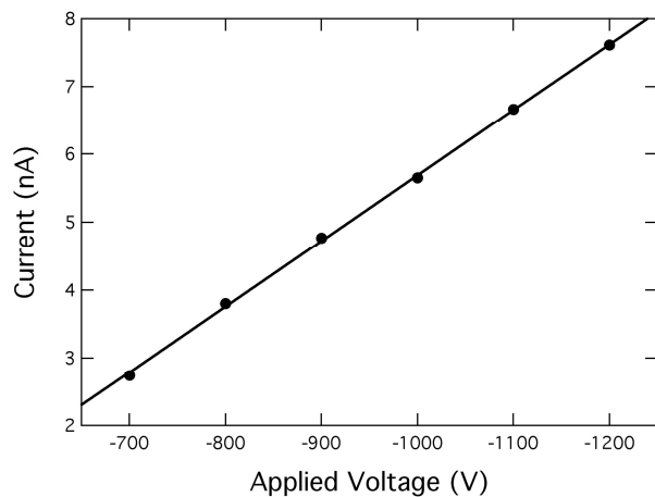
Fig. 4. The current is measured as a function of the applied voltage. The pressure of helium gas is 3 torr. The magnitude of the current corresponds to the efficiency of helium ionization. The line in the figure came from the linear fitting of the data. The ionization current of helium gas linearly increased as the voltage that was applied to the cathode increased.
