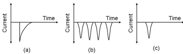
Fig. 2. Typical shapes of pulses from a tungsten tip. (a), (b), and (c) represent the typical shapes of a pulse at 500, 3, and 0.001 torr, respectively. The pulses were measured with an oscilloscope when the voltage that was applied to the tip was -1,200 V. The asymmetrical shape of the pulse in (a) shows that the electrons that were emitted from the tip collided much with the helium atoms due to the high pressure. The many symmetrical shapes of the pulses in (b) show that the electrons that were emitted from the tip ionized the helium atoms very efficiently, and the symmetric shape of the pulse in (c) shows that the electrons that were emitted from the tip did not ionize the helium atoms much due to the low density of helium gas, even when the electron energy was high enough to ionize helium.
