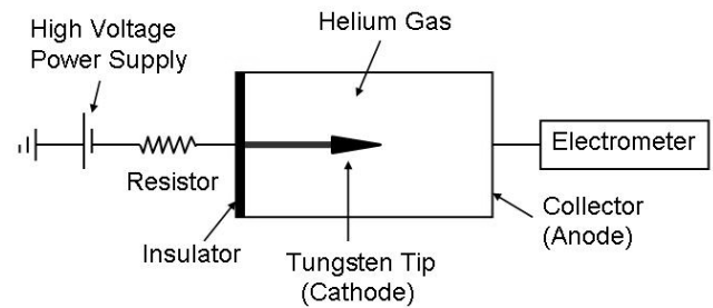
Fig. 1. Apparatus for measuring helium ionization. To protect the tungsten tip from ohmic heating, a 100\text{-G}\Omega resistor was connected to the field emission tip. A collector made of copper was used to measure the current with an electrometer. The tungsten tip and the collector corresponded to the negative electrode and the positive electrode, respectively. The distance between the field emission tip and the collector was 1 cm.
