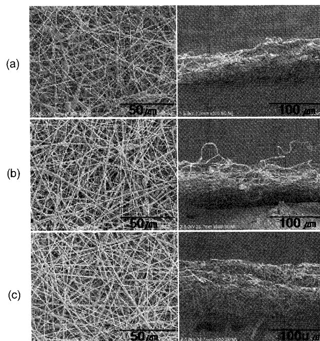
Figure 2. SEM images of electrospun fibers and thickness of fabricated mats: (a), (b), and (c) numbers are the fabricating conditions of the electrospun mats, which were described in Table 1.
