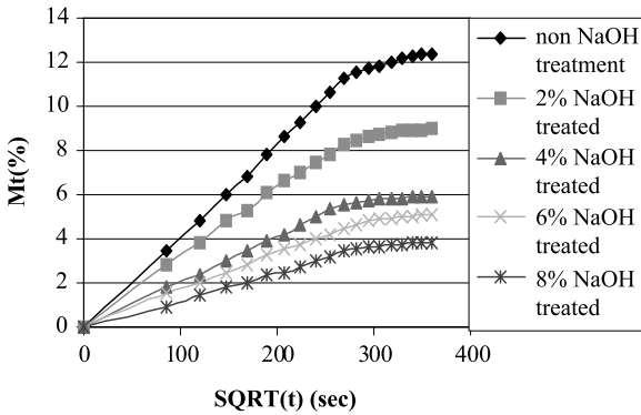
Figure 12. Water absorption on coir/PP composites.
