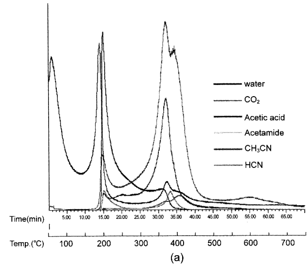
Figure 9. TD-MSD TIC of PAAA and CdS/PAAA.
