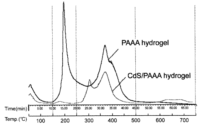
Figure 9. TD-MSD TIC of PAAA and CdS/PAAA.
