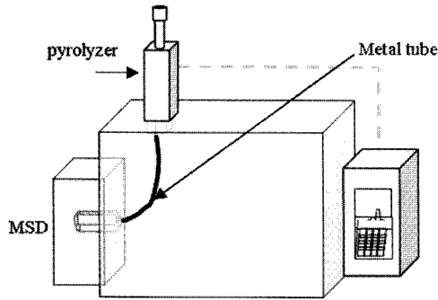
Figure 4. Equipment for TD-MSD experiment.
