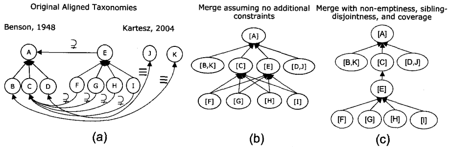
Figure 6. Merging Ranunculus Hispidus under Different Assumptions. For Clarity, the Disjointness Relations between Taxa in (c) are not Shown. See Text for Further Detail.
