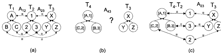
Figure 3. Using the Projection.
