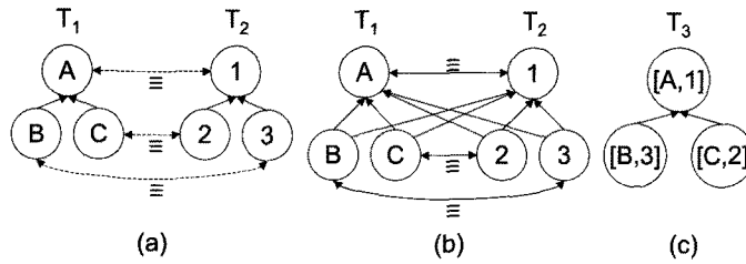
Figure 4. Merging with and Without Fusing Equivalent Taxa.
