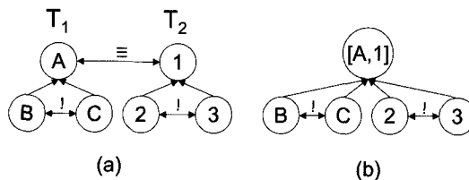
Figure 7. Constraints Placed on Taxonomies before the Merge May not Apply to the Result of the Merge.
