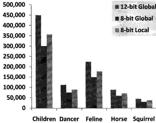
Figure 8. Compressed data sizes with different quantization methods.
