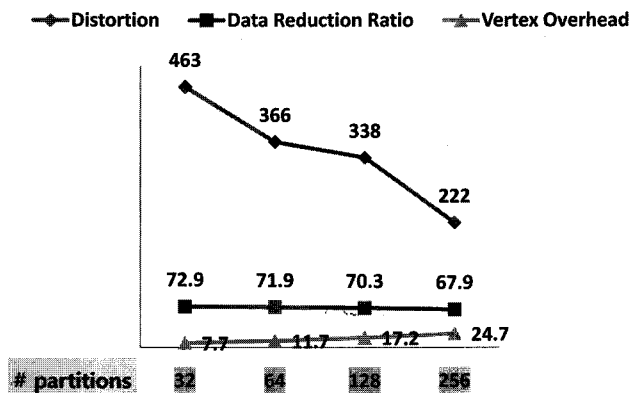
Figure 7. Compression results with different numbers of partitions for dancer model. Distortions are shown in the unit of 10^{-6} .
