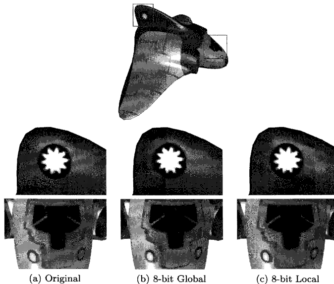
Figure 10. Comparison of texture mapping result between 8-bit global and 8-bit local quantization of texture coordinates.
