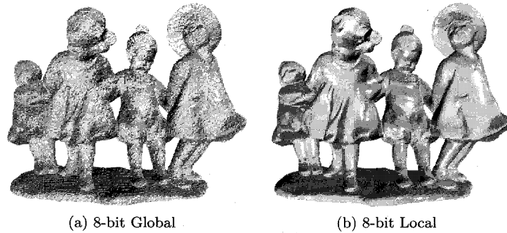
Figure 9. Visual quality comparison between 8-bit global and our 8-bit local quantization.
