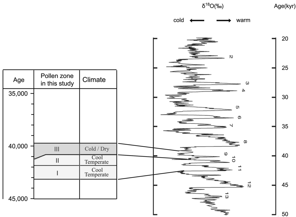
Fig. 5. Comparison of Uiwang pollen record with oxygen isotope record from Greenland (Dansgaard et al., 1993).
