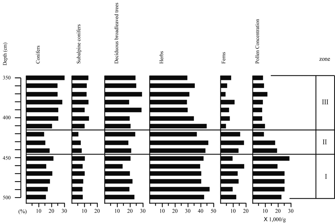
Fig. 4. Fluctuation in proportions of fern spores, coniferous pollen, subalpine coniferous pollen, pollen of deciduous broadleaved trees and herbaceous pollen.
