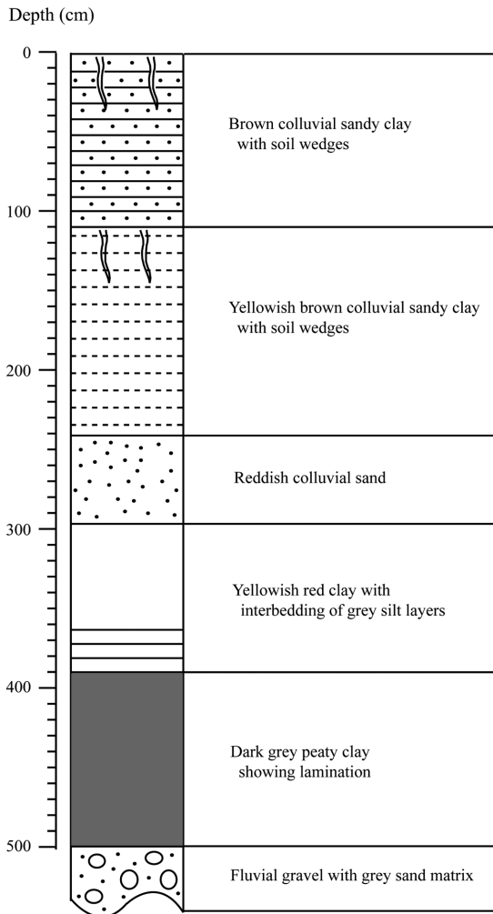
Fig. 2. Lithology of the 5 m-thick section studied.
