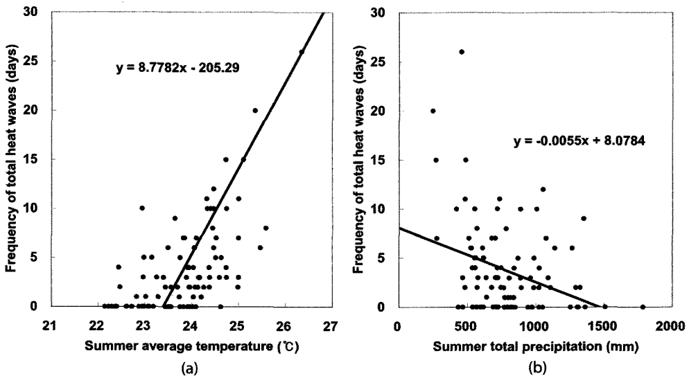
Figure 4. Sensitivity of occurrences of heat wave days to summer average temperature (a) or to summer total precipitation (b) in Seoul, 1907-2008. The regression lines indicate the first eigenvector of the principal component analyses that considers bidirectional errors for both x and y variables. 서울의 여름철 평균기온(a) 또는 총 강수량(b)에 대한 열파일 발생의 민감도(1907~2008).
